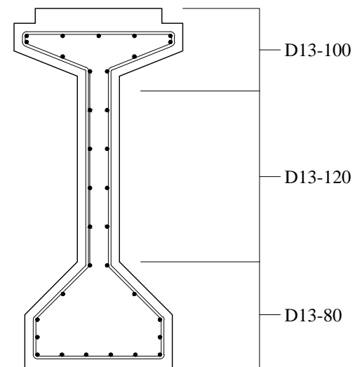
DETAIL TULANGAN NON-PRATEGANG
