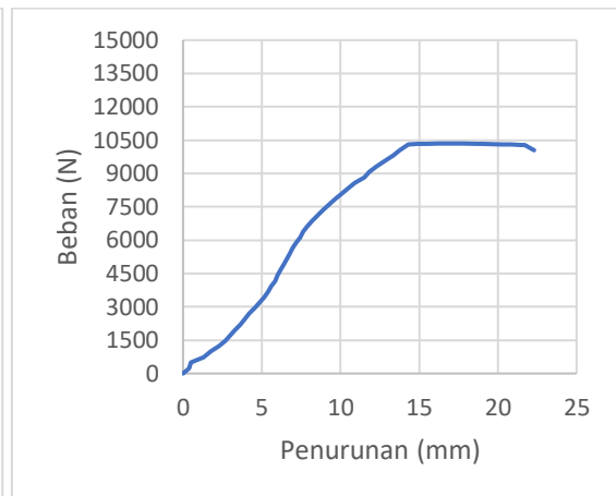
Grafik 8.14 Pengujiuan KS-12mm-1
