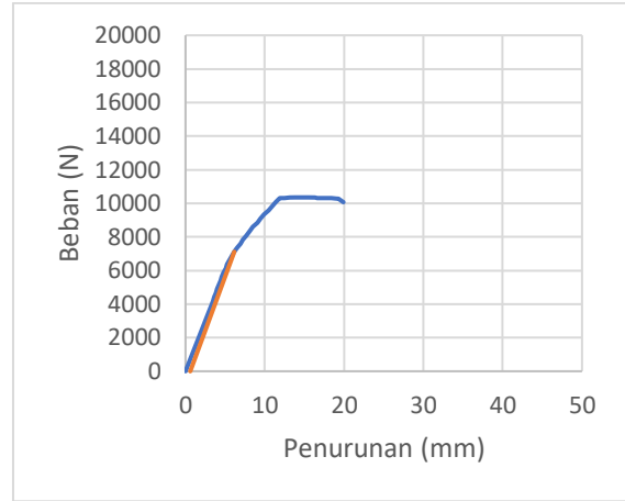
Grafik 14.14 KS-12mm-1 Terkoreksi
