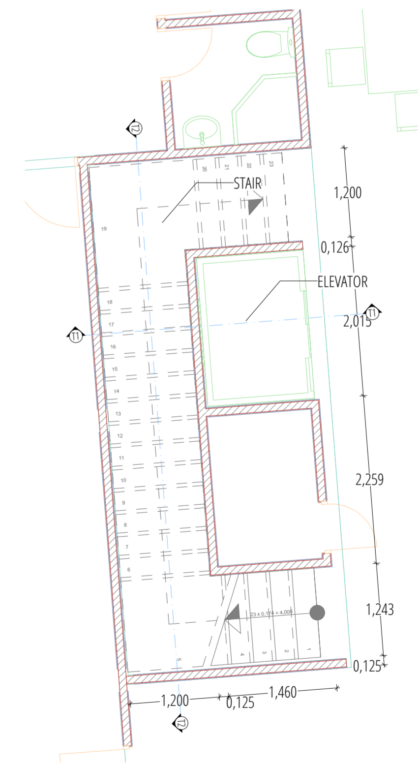
07-03 - STAIR & ELEVATOR DETAIL 1:50
