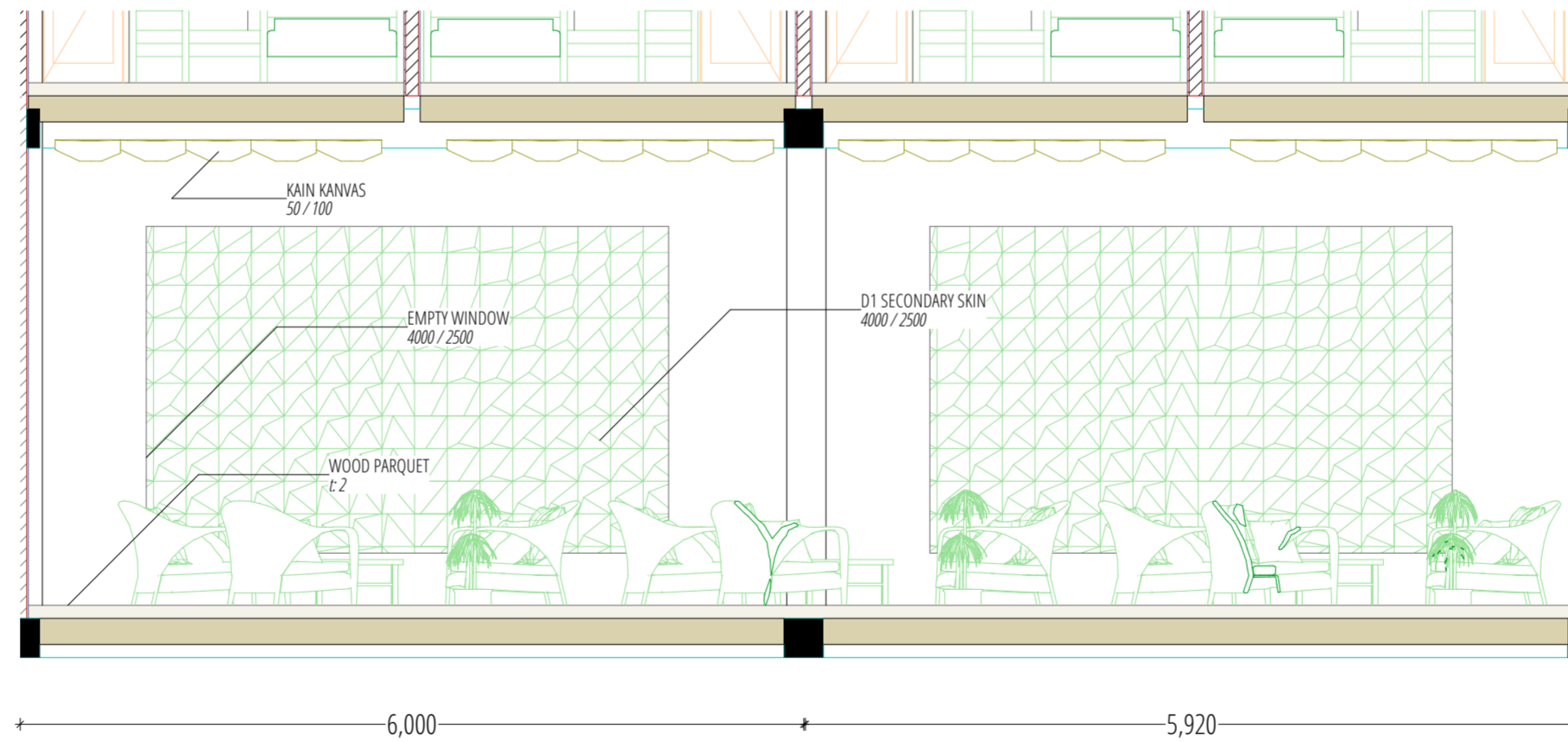
LIVING ROOM ELEVATION 1:50
