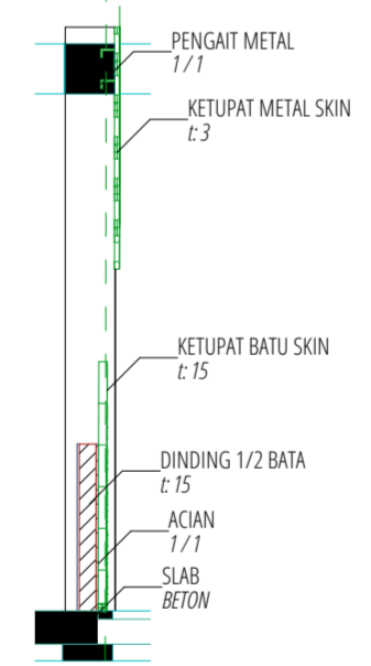
08-02 - D2 SECTION DETAIL 1:50
