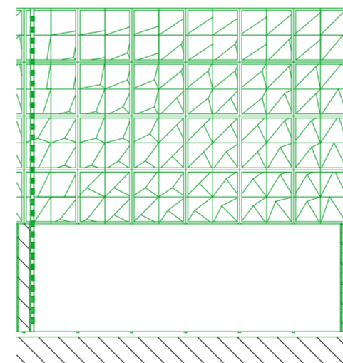
08-01 - D1" BACK ELEVATION DETAIL 1:50
