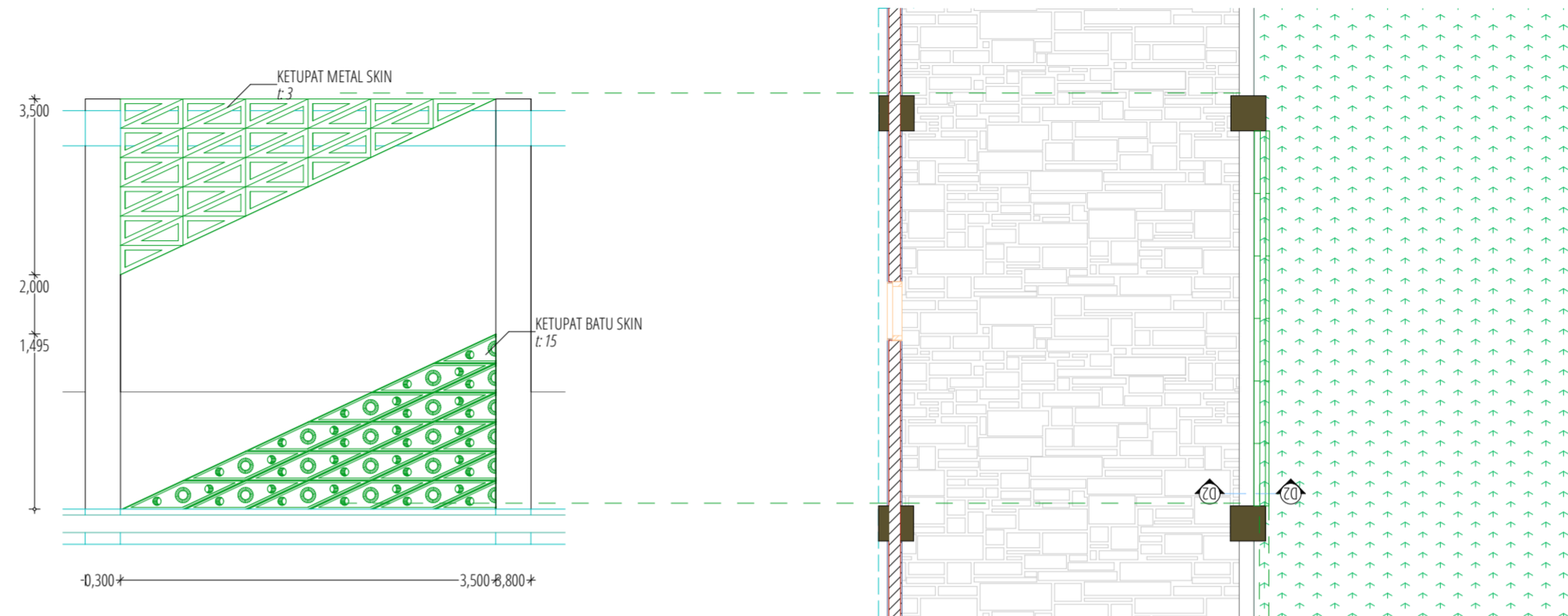
08-02 - FRONT ELEVATION DETAIL 1:50
