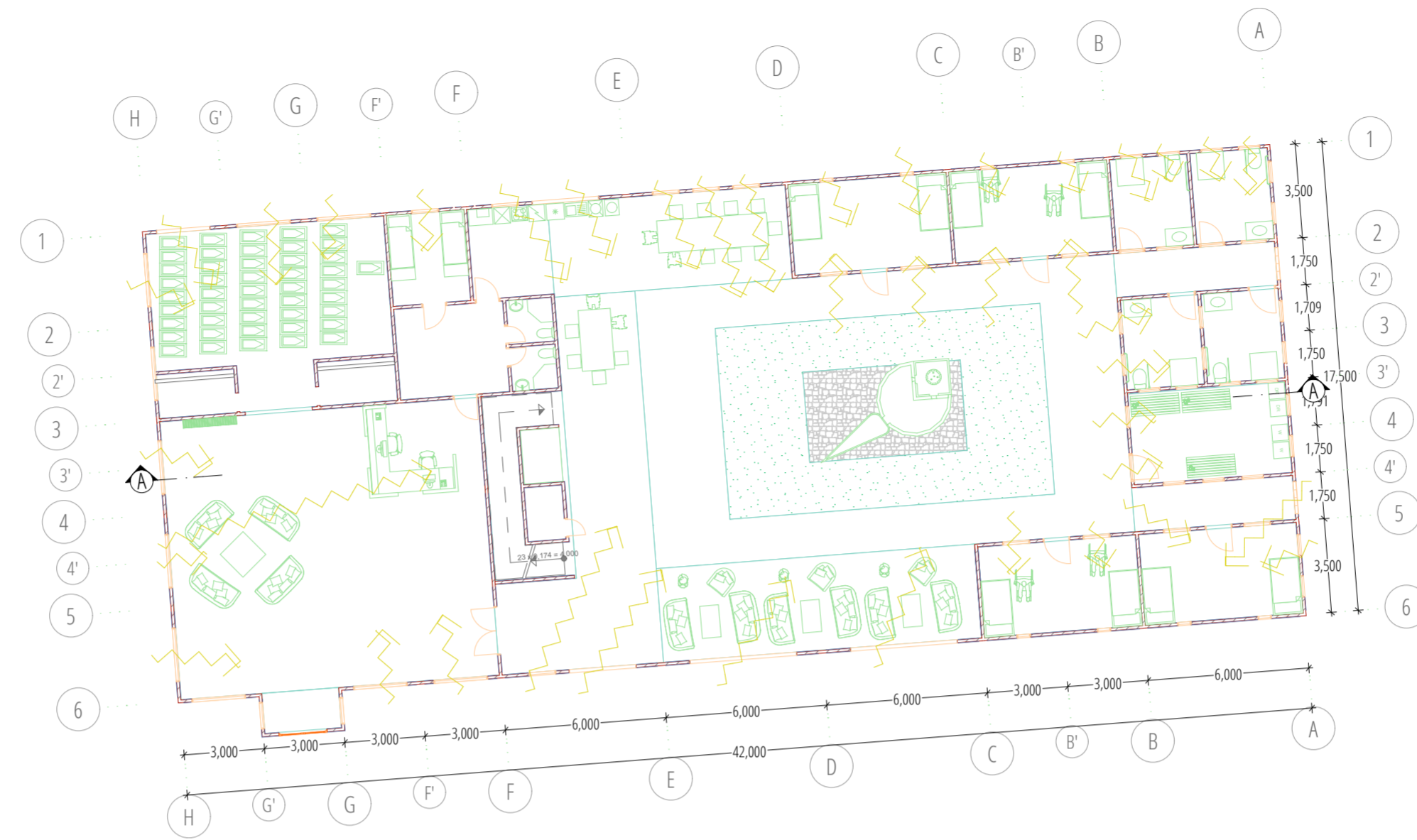
GF NATURAL LIGHTING PLAN 1:200
