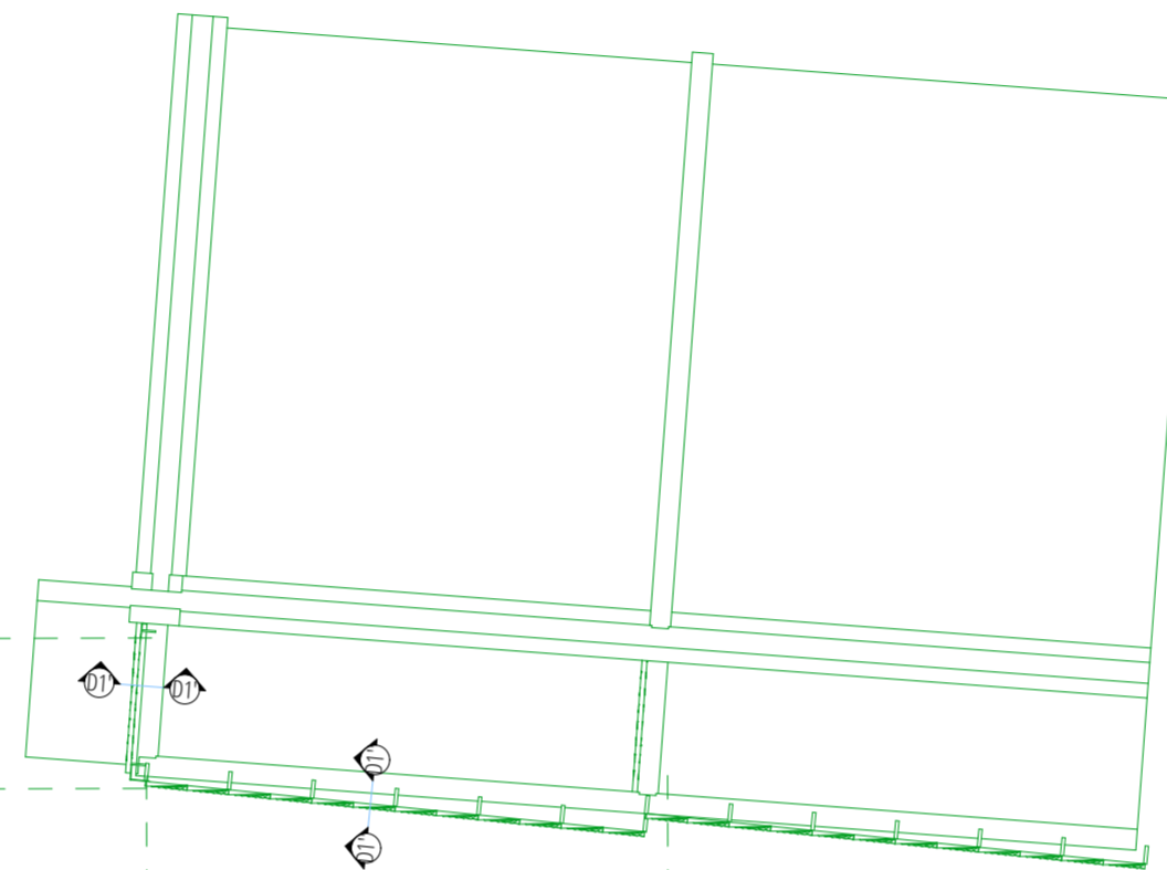
08-01 - BALCON 2NDARY SKIN PLAN DETAIL 1:50
