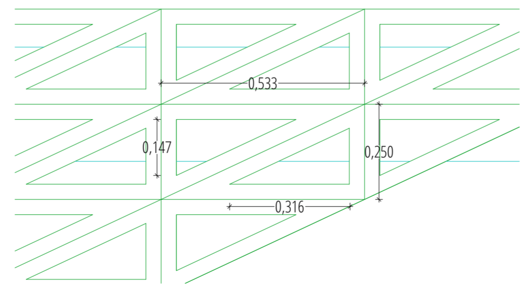
08-02 - KETUPAT DETAIL 1:10
