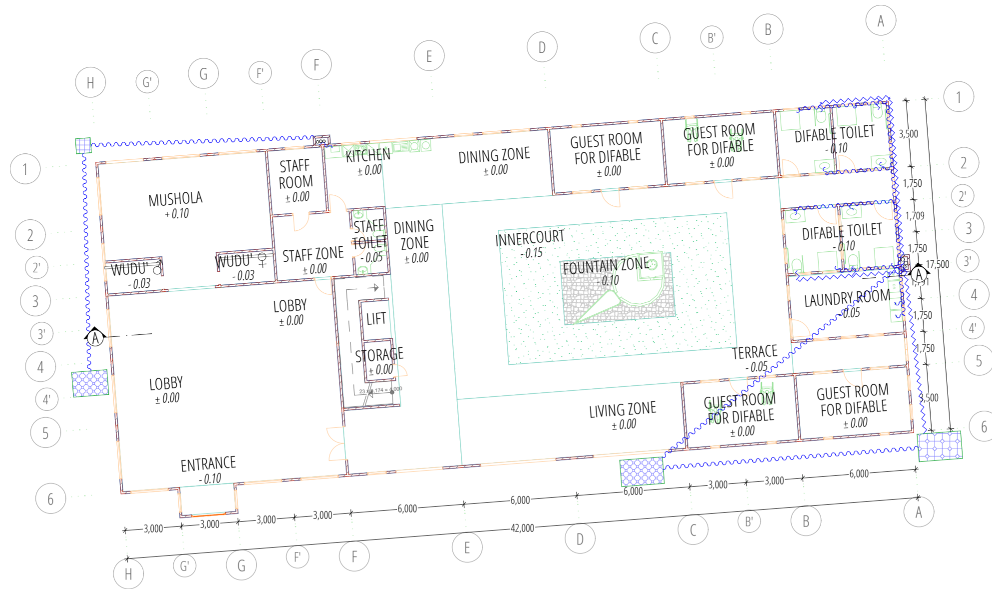
GF GREY WATER PLAN 1:200
