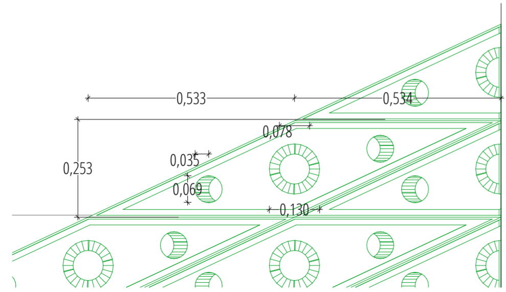
08-02 - KETUPAT DETAIL 1:10
