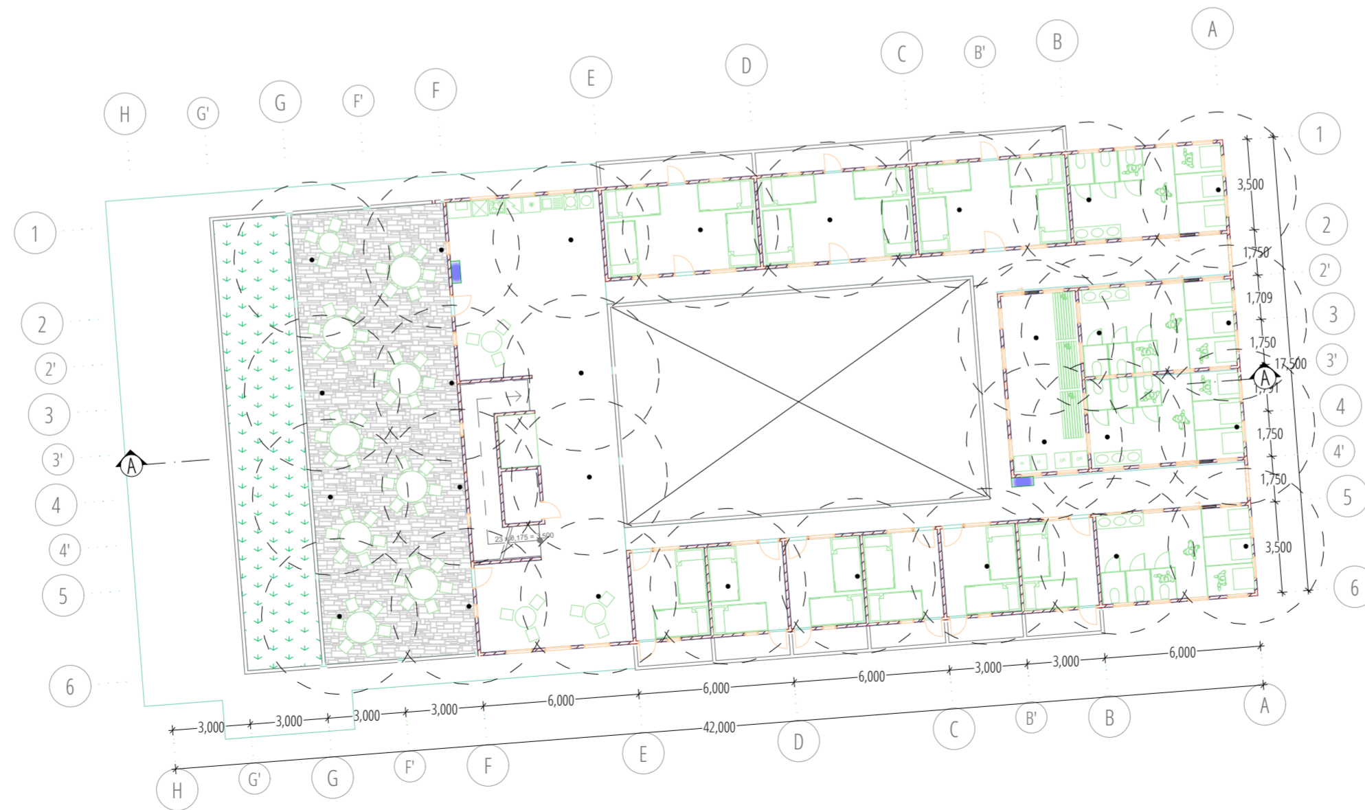
1ST FLOOR FIRE PROTECT PLAN 1:200
