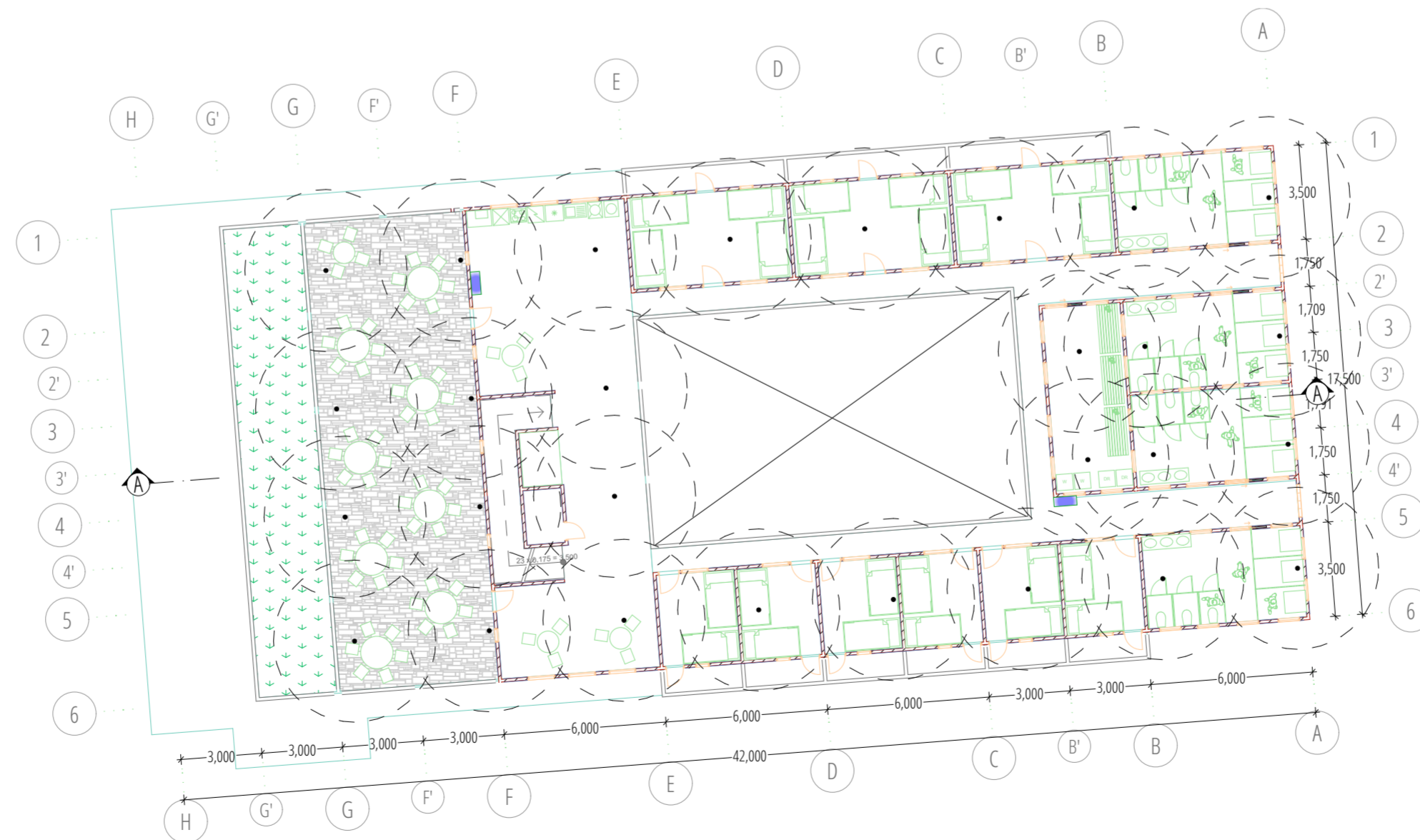
1ST FLOOR NATURAL VENTILATION PLAN 1:200
