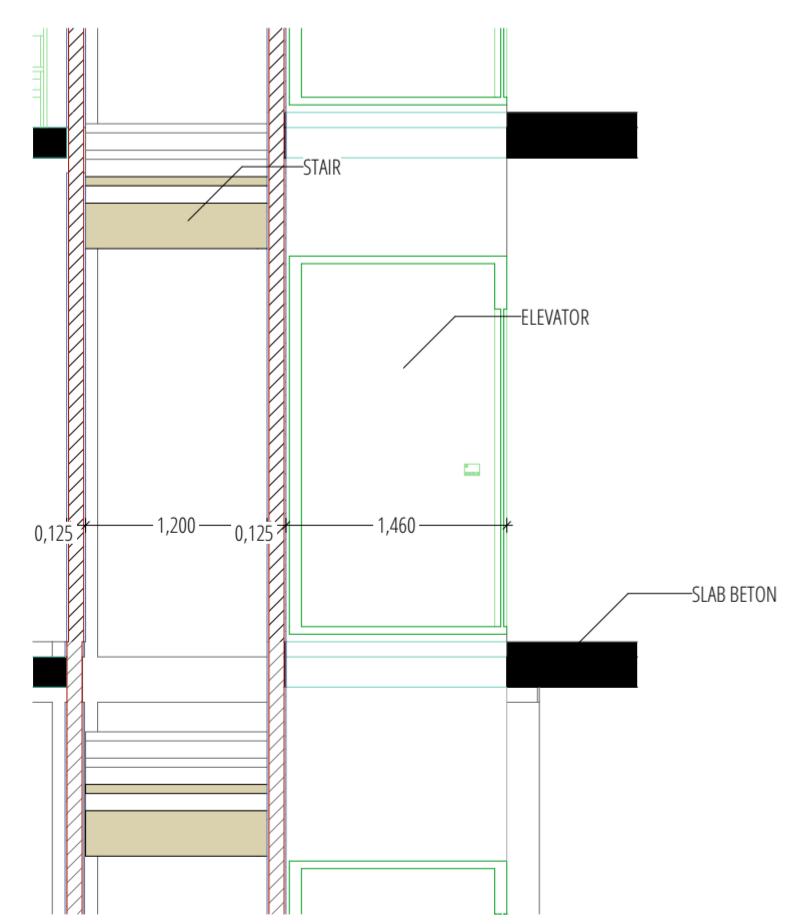
07 03 - T1 VERTICAL TRANSPORTAION SECTION 1:50
