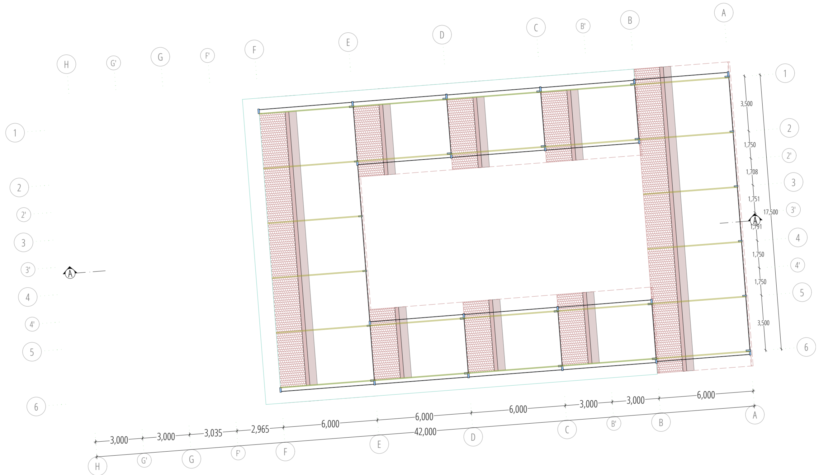
ROOF TOP PLAN 1:150
