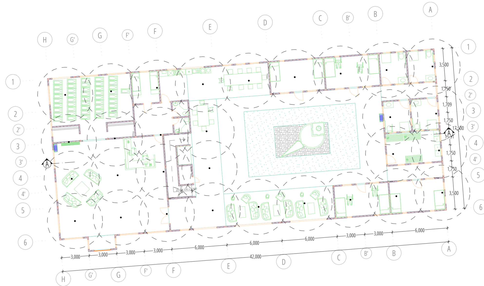
GF NATURAL VENTILATION PLAN 1:200
