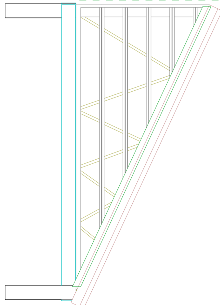
10 - ROOF SIDE ELEVATION DETAIL 1:50
