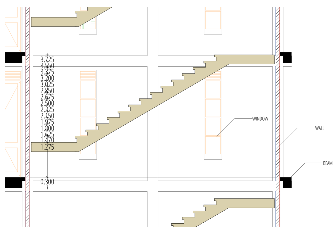
07 03 - T2 VERTICAL TRANSPORTAION SECTION 1:50
