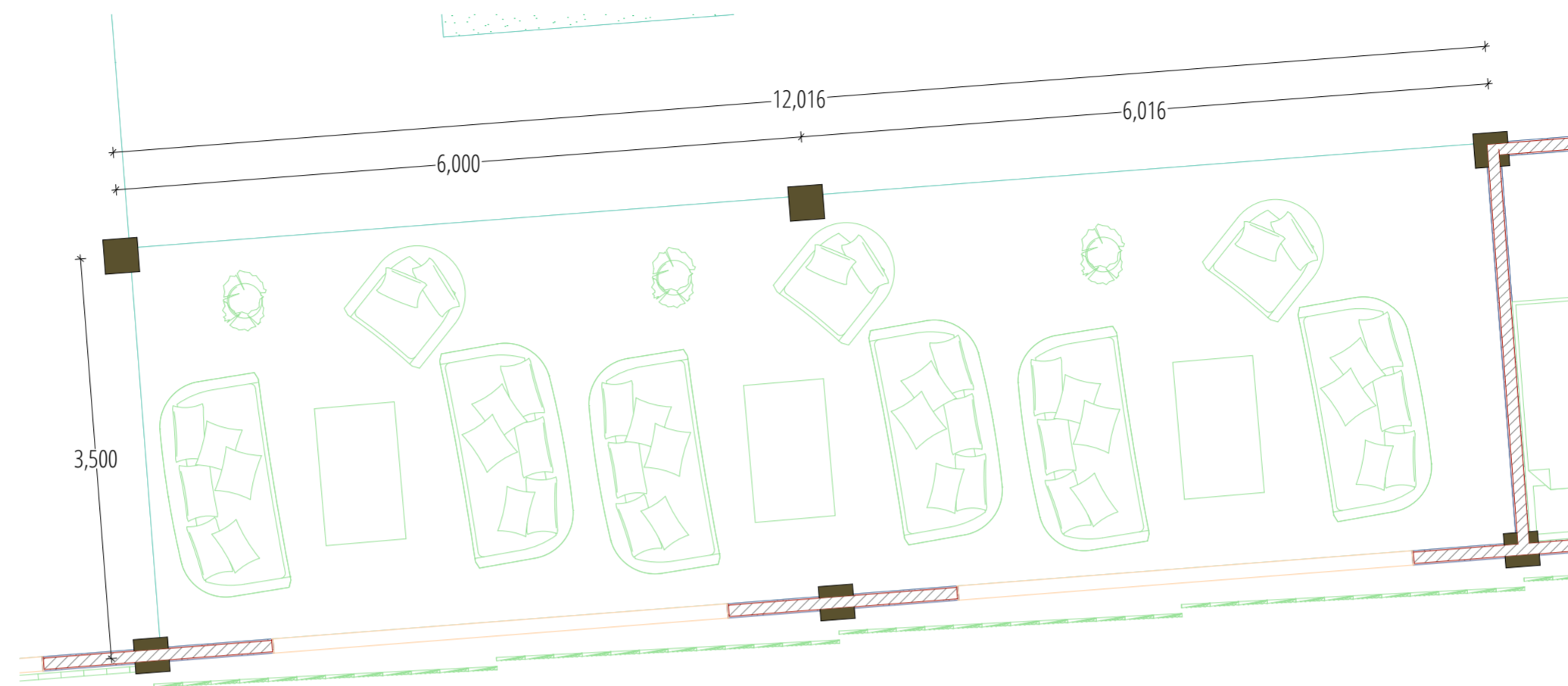
LIVING ROOM PLAN DETAIL 1:50
