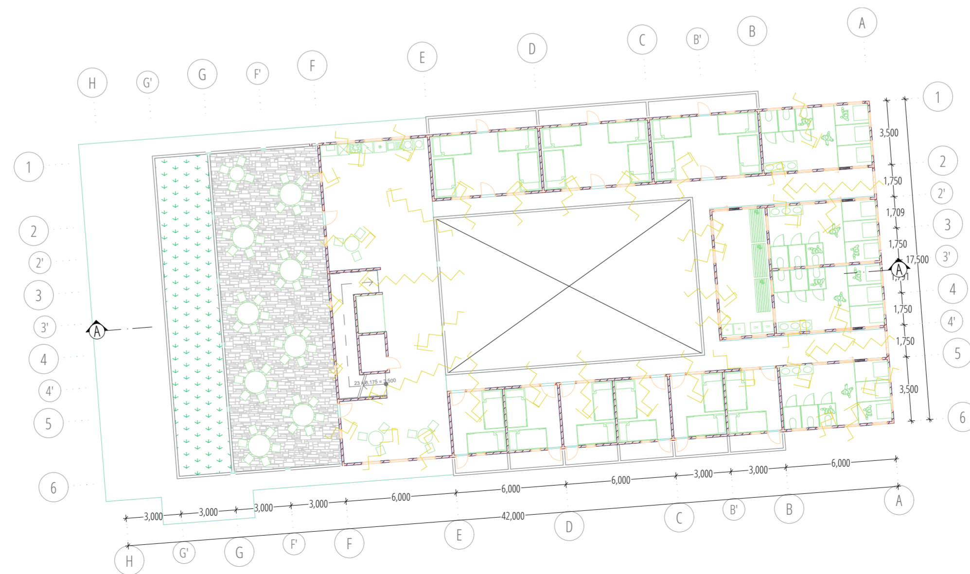
1ST FLOOR NATURAL LIGHTING PLAN 1:200
