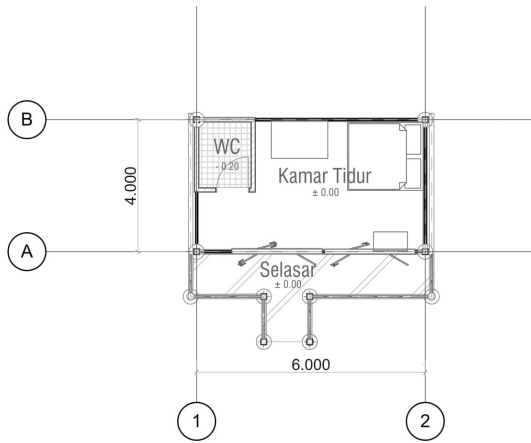
DENAH BUNGALOW RESORT 1 Skala 1 : 100
