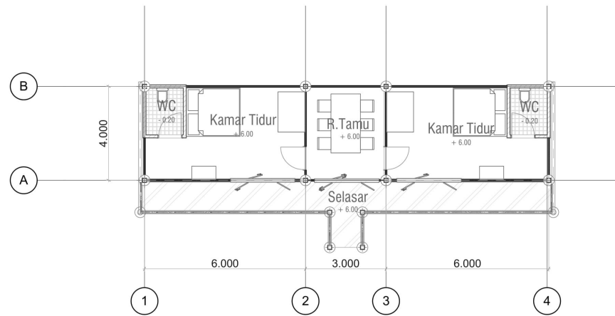
DENAH BUNGALOW RESORT 2 Skala 1 : 100
