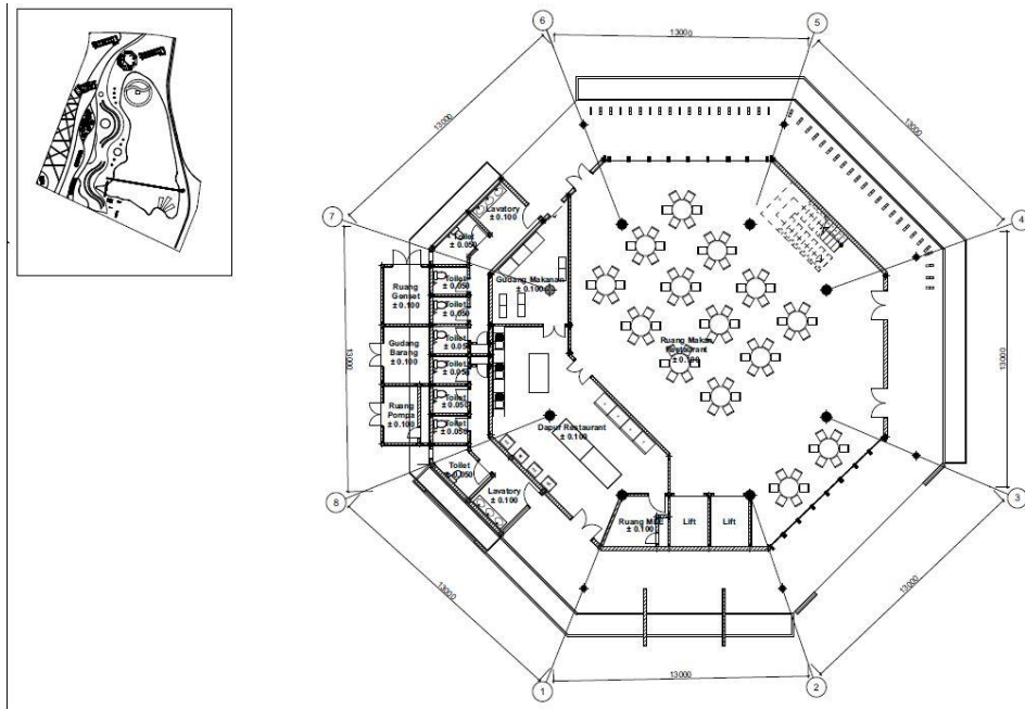
Gambar 7. 2 Redesign denah Restaurant dan Indoor Outbound
