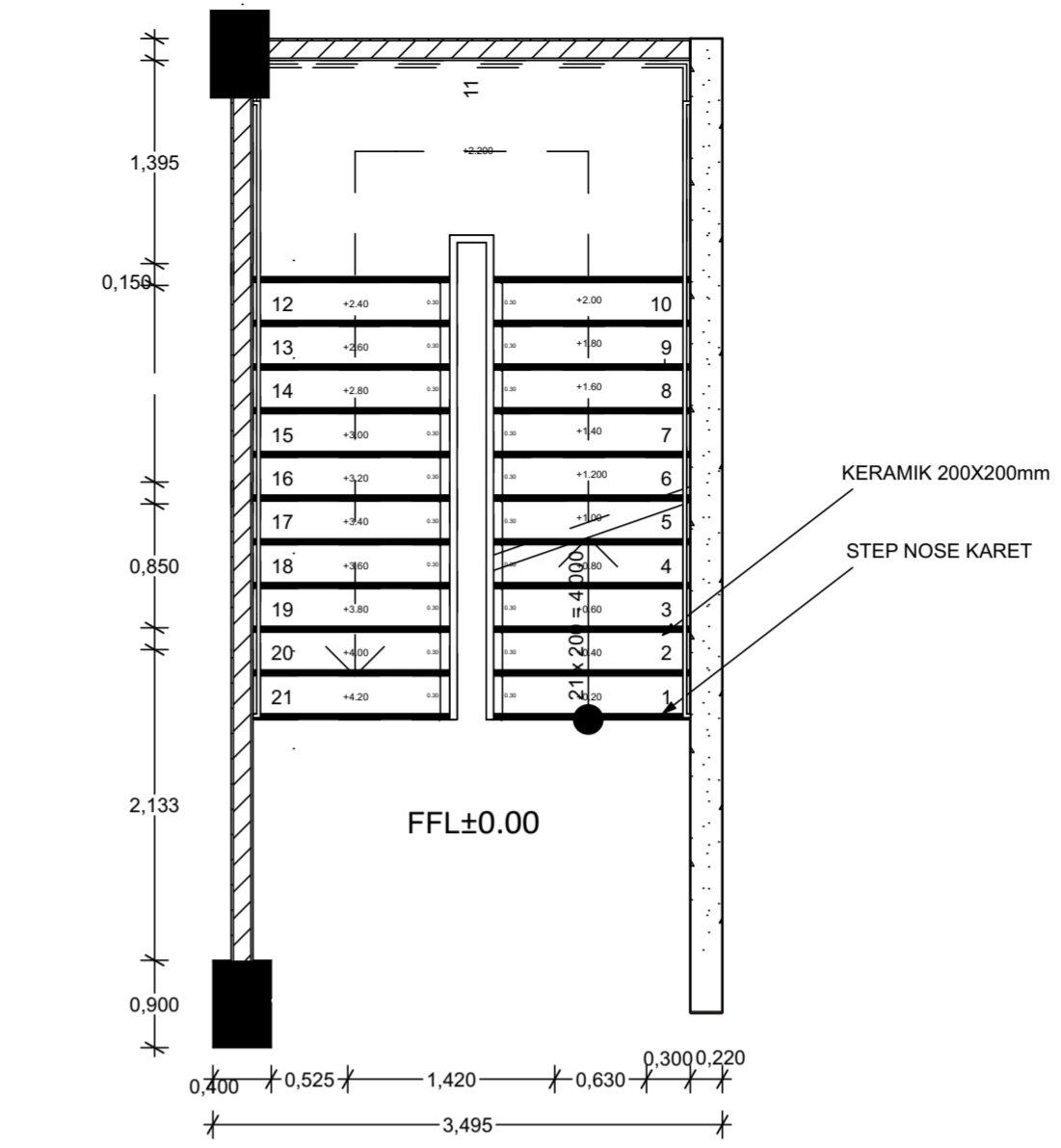
MAIN STAIRS PLAN SCALE 1:50
