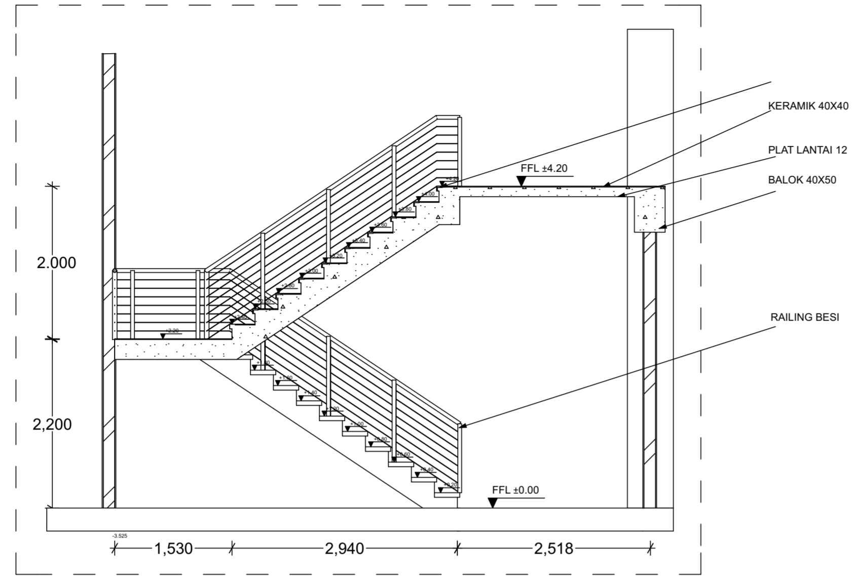
MAIN STAIRS SECTION SCALE 1:50
