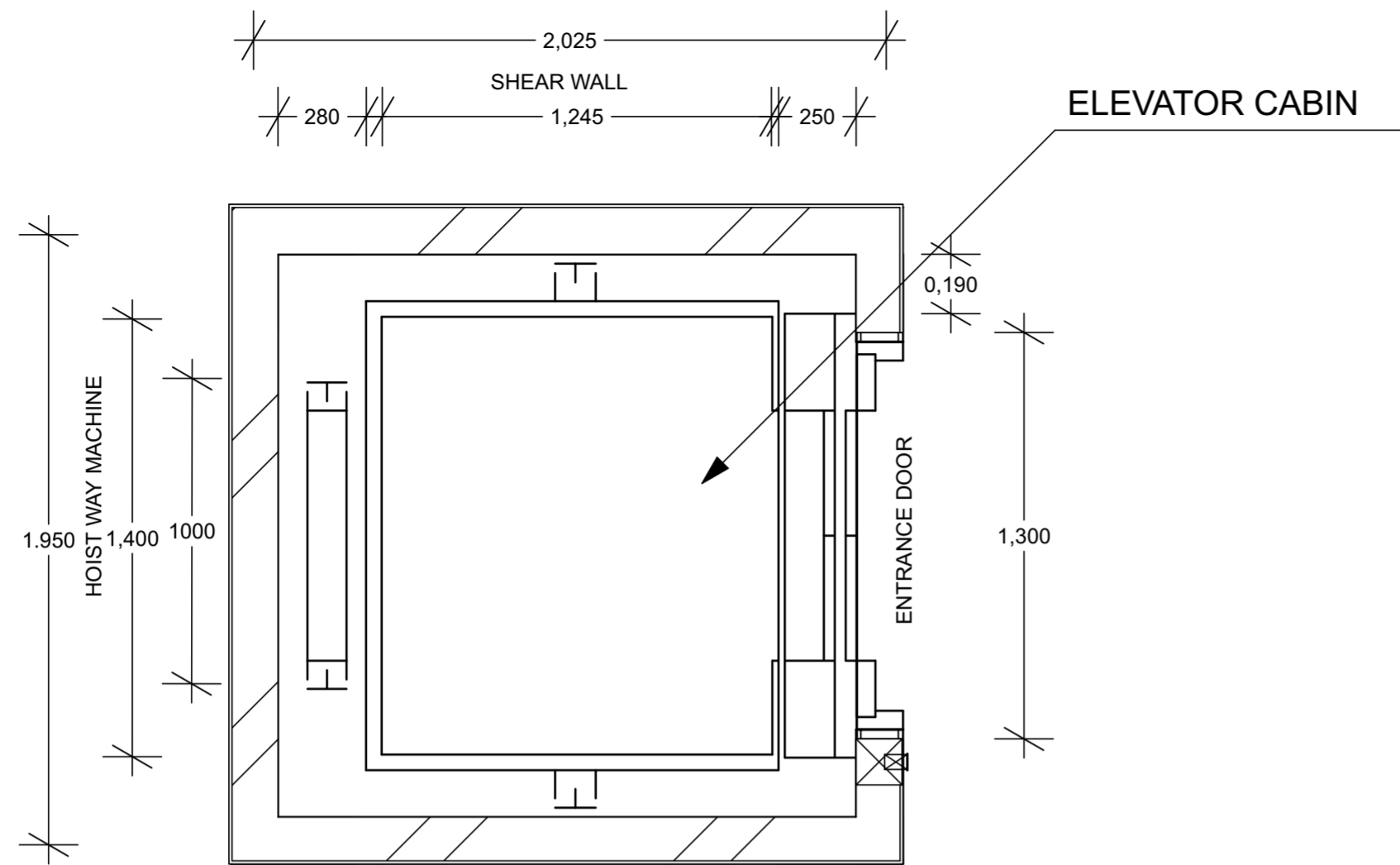
PASSENGER ELEVATOR PLAN SCALE 1:20
