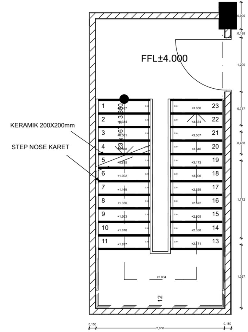
EMERGENCY STAIRS SCALE 1:50
