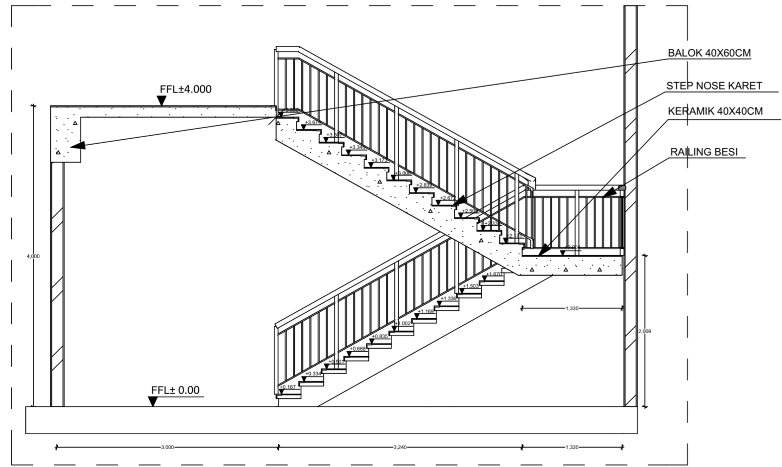
EMERGENCY STAIRS SECTION SCALE 1:50
