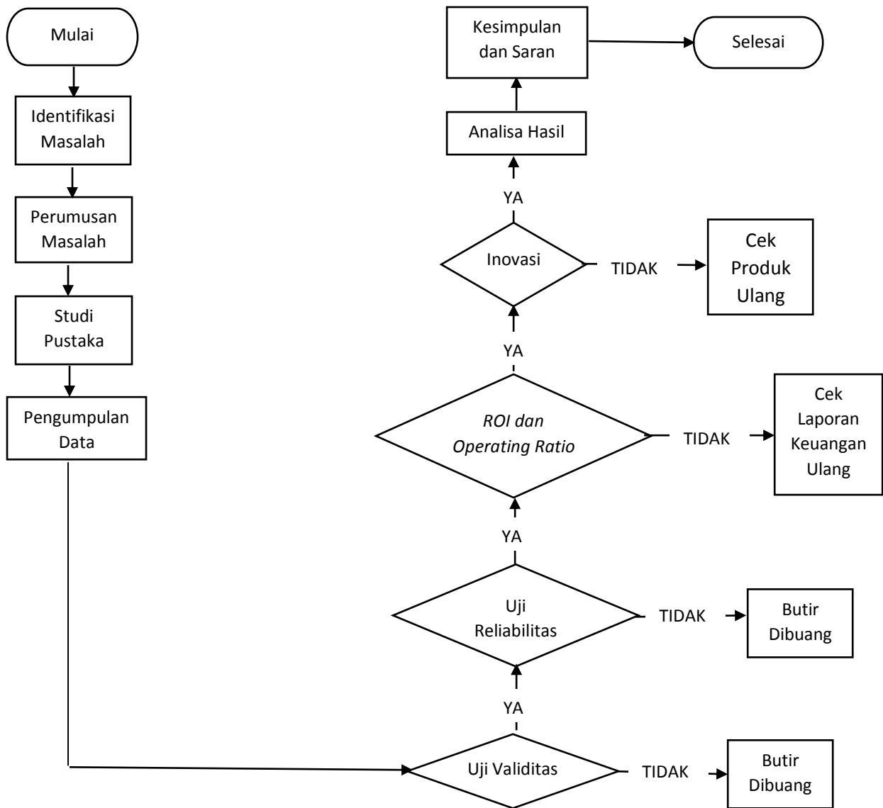
Gambar 3.1 Flowchart
