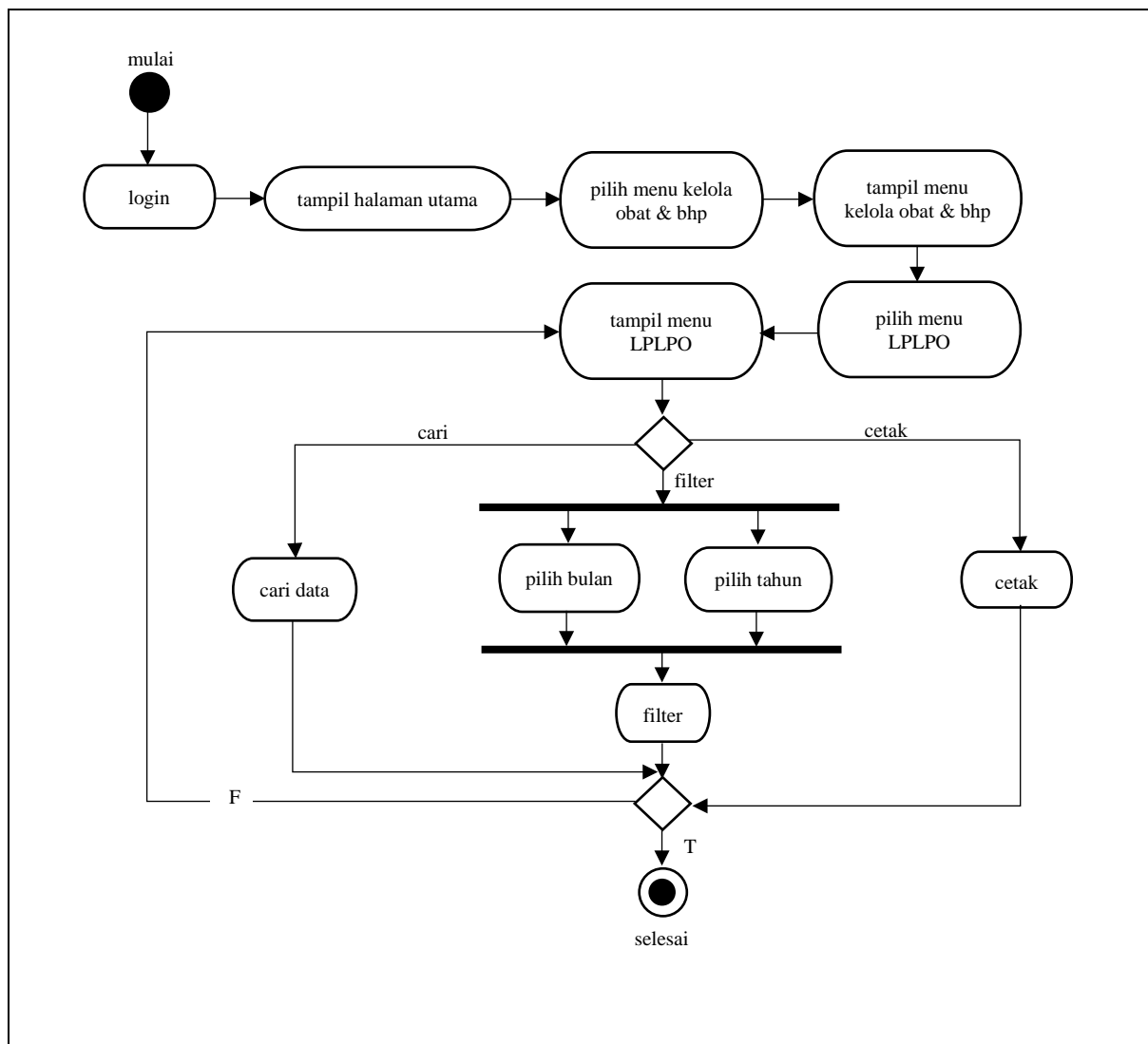
Gambar 3.10 Activity Diagram LPLPO
