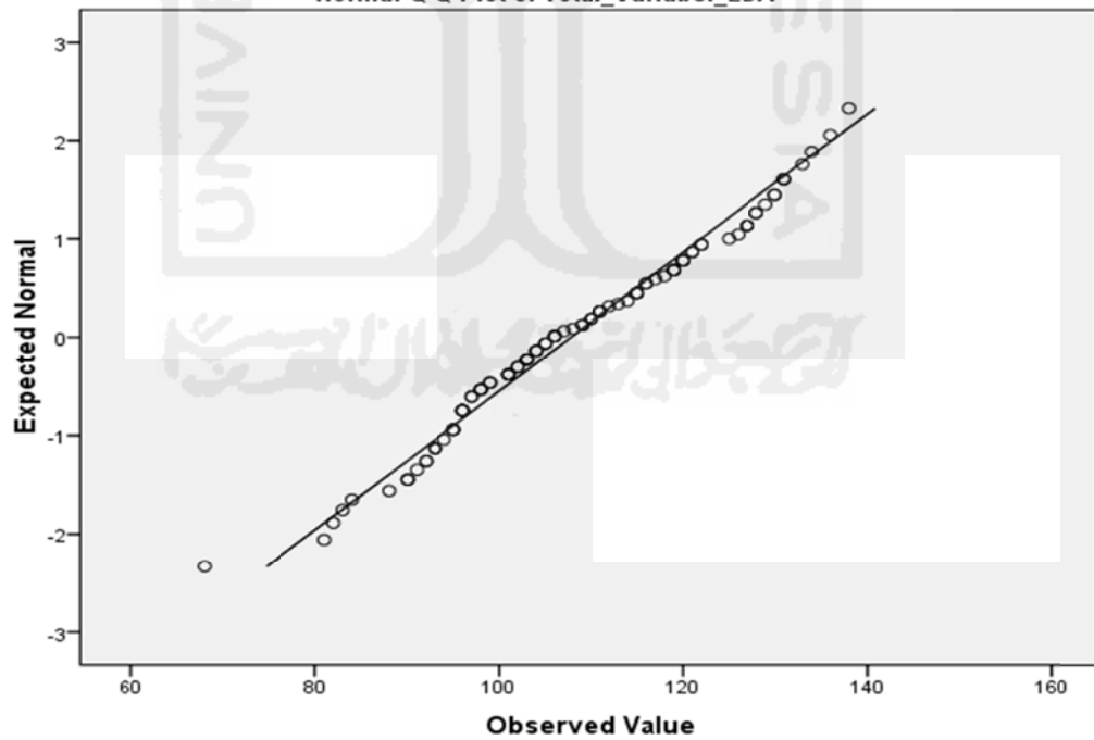
Normal Q-Q Plot of Total_Variabel_EDA
