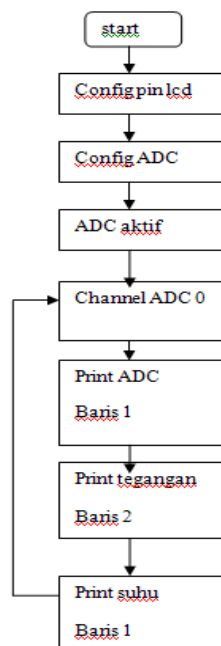
Gambar 3. 22 Flowchart ADC
