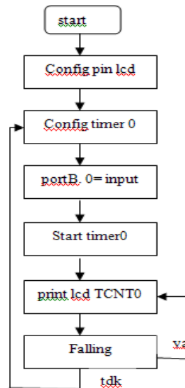
Gambar 3. 19 Flowchart Counter
