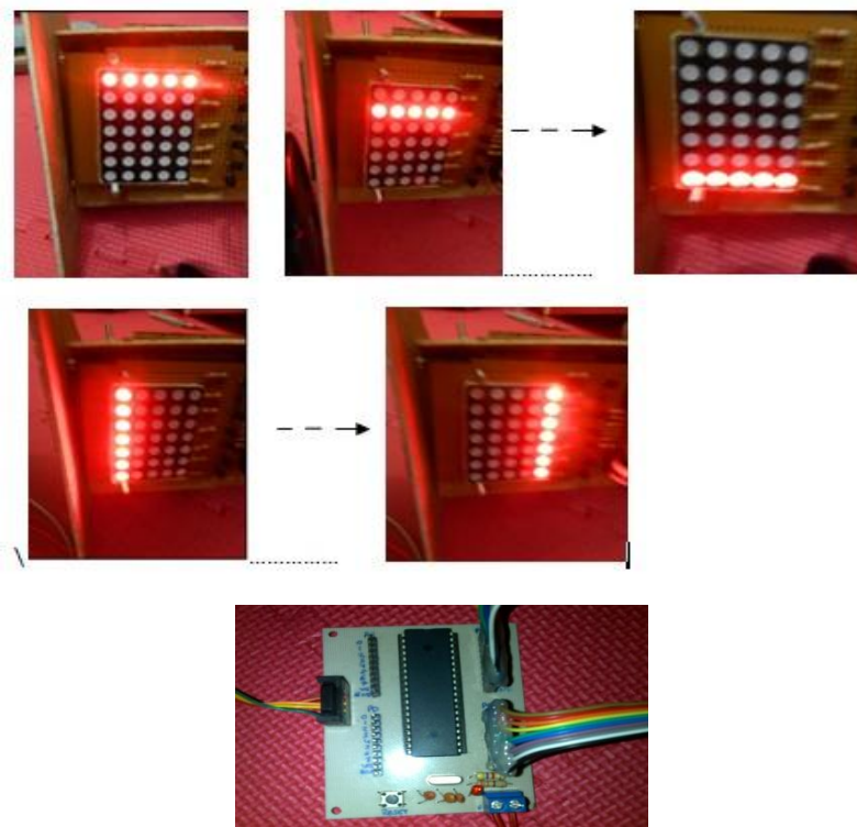
Gambar 4. 9 Dotmatrik
