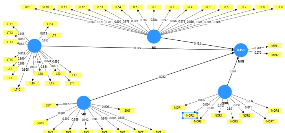
Gambar 4.2 Model Output Outer Model
