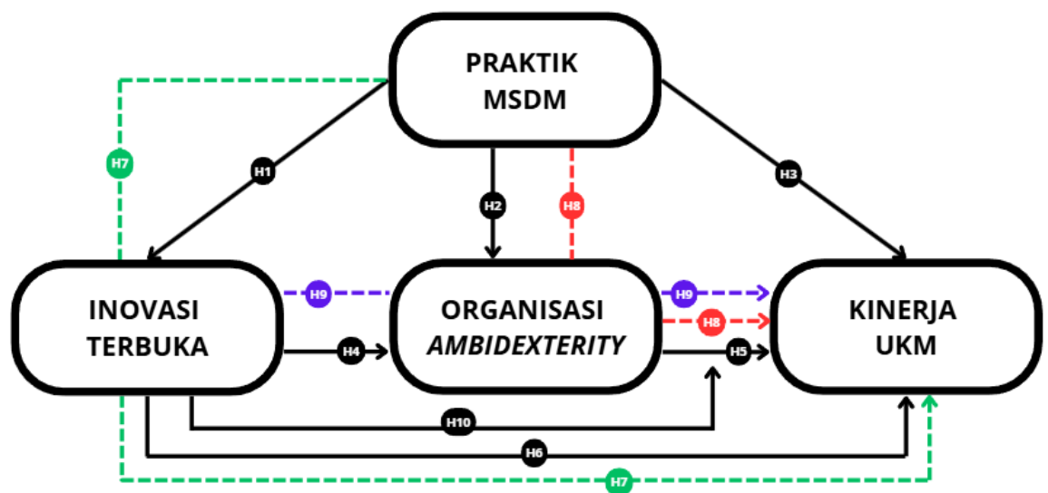
Gambar 2. 1 Model Empiris
