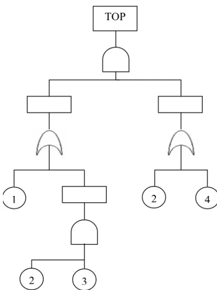
Gambar 1 Contoh Fault Tree Analysis
