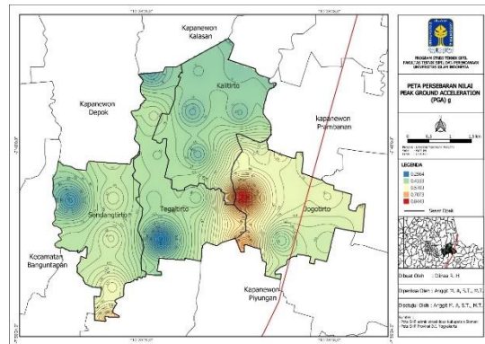
Gambar 14. Peta Persebaran Nilai Peak Ground Acceleration (PGA) g
