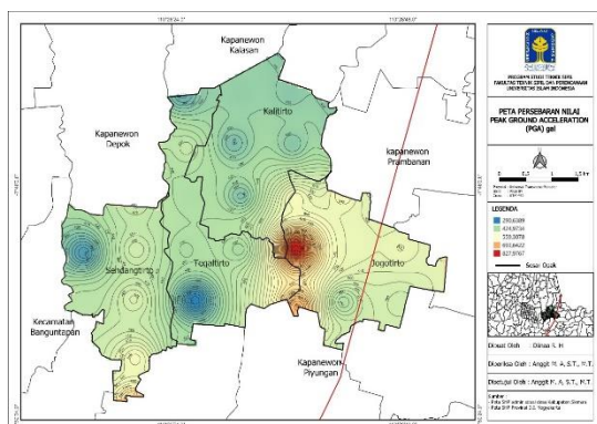
Gambar 13. Peta Persebaran Nilai Peak Ground Acceleration (PGA) gal
