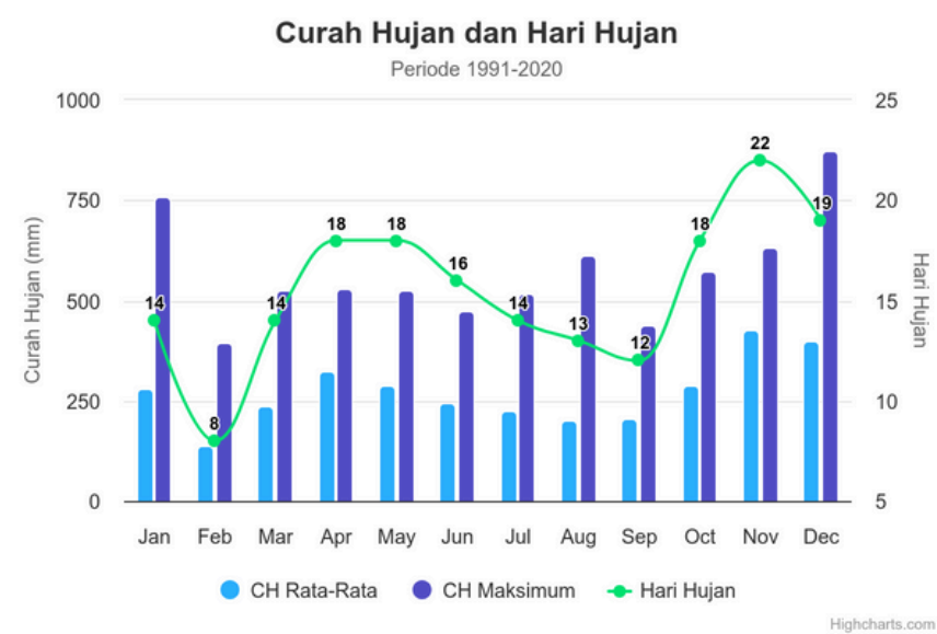
Gambar 17.0 Data curah hujan Sumber : https://www.meteoblue.com
