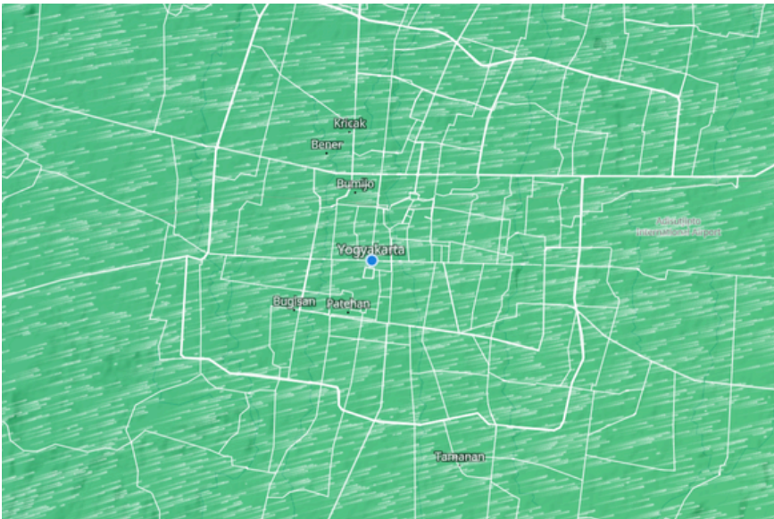
Gambar 18.0 Data arah angin Sumber : https://www.meteoblue.com
