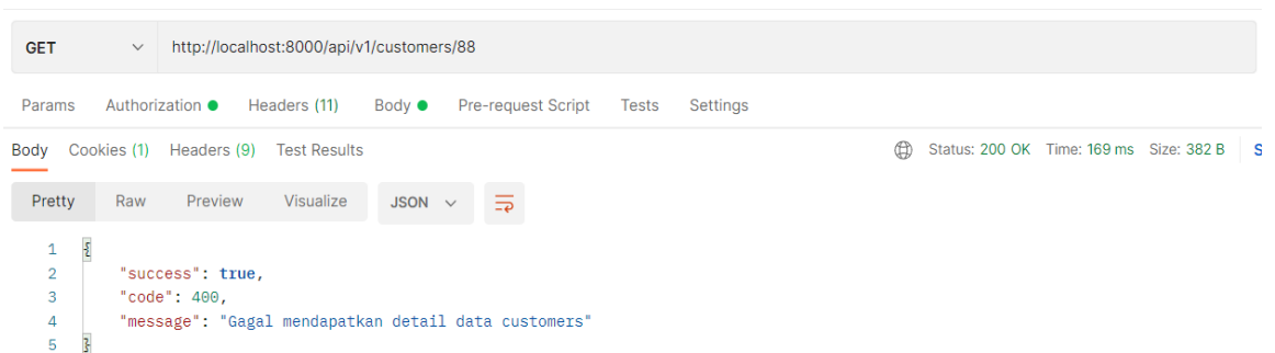
Gambar 3.16 Response Melihat Detail Data Customer Berhasil.
