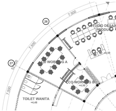
Gambar 4.87 Detail Denah Co Working Sumber : Penulis, 2023
