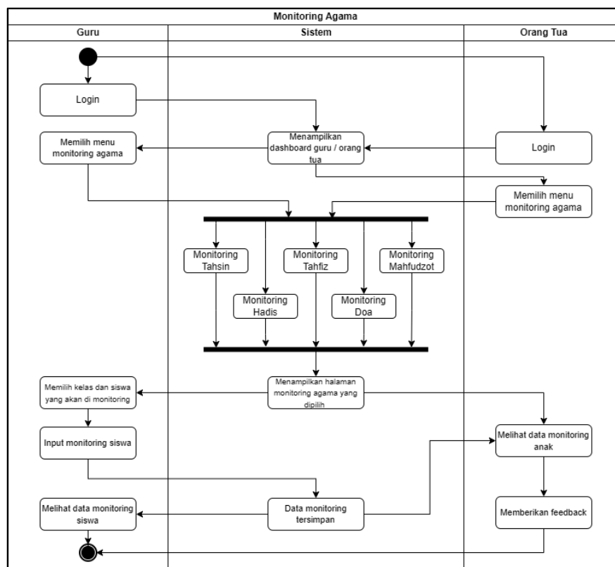
Gambar 4.2 Activity Diagram Monitoring Agama
