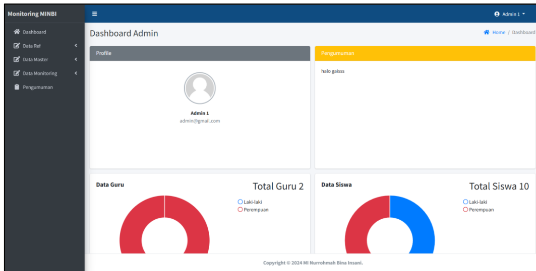
Gambar 4.14 Dashboard Admin
