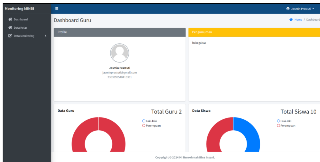
Gambar 4.33 Dashboard Guru
