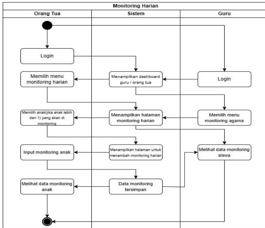
Gambar 4.3 Activity Diagram Monitoring Harian
