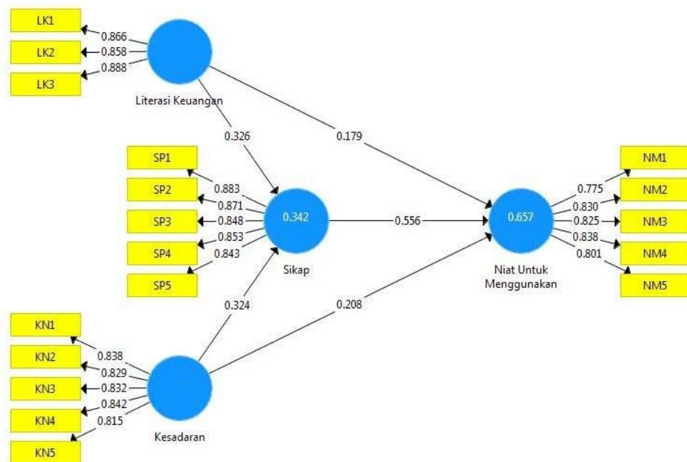
Gambar 4.1 Model Struktural
