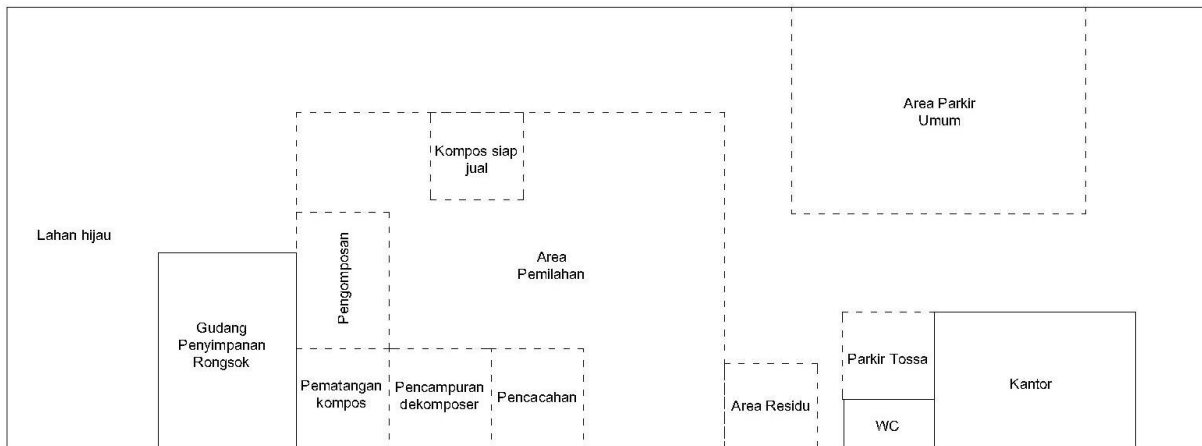
Gambar 4.2 Denah TPS 3R Ben Resik
