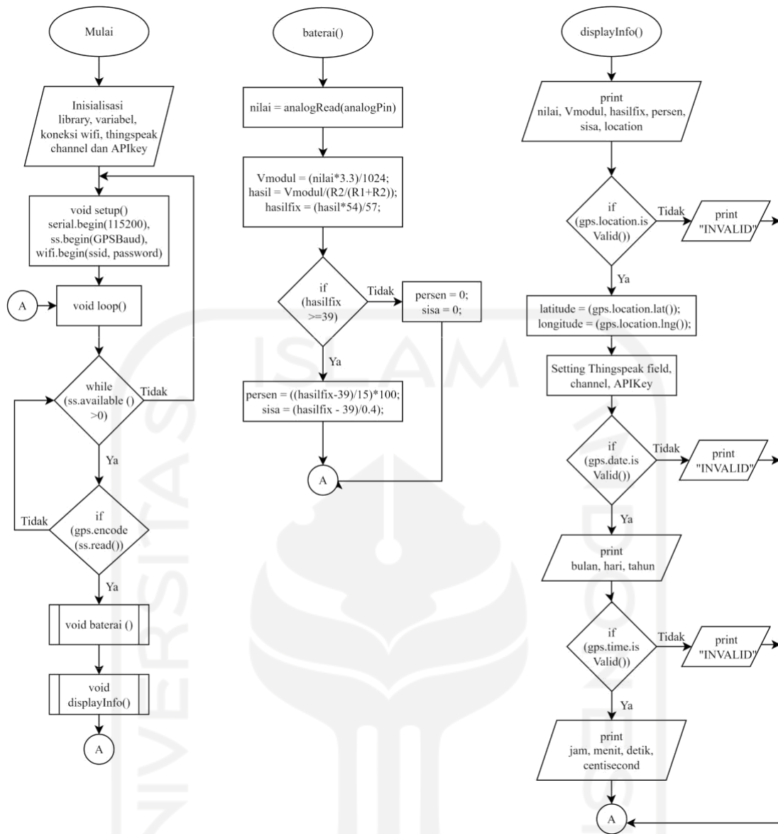
Gambar 3.5. Flowchart program
