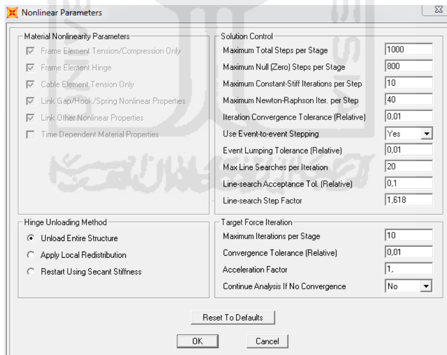
Gambar 5.34 Load case data – nonlinear static GRAVITASI
