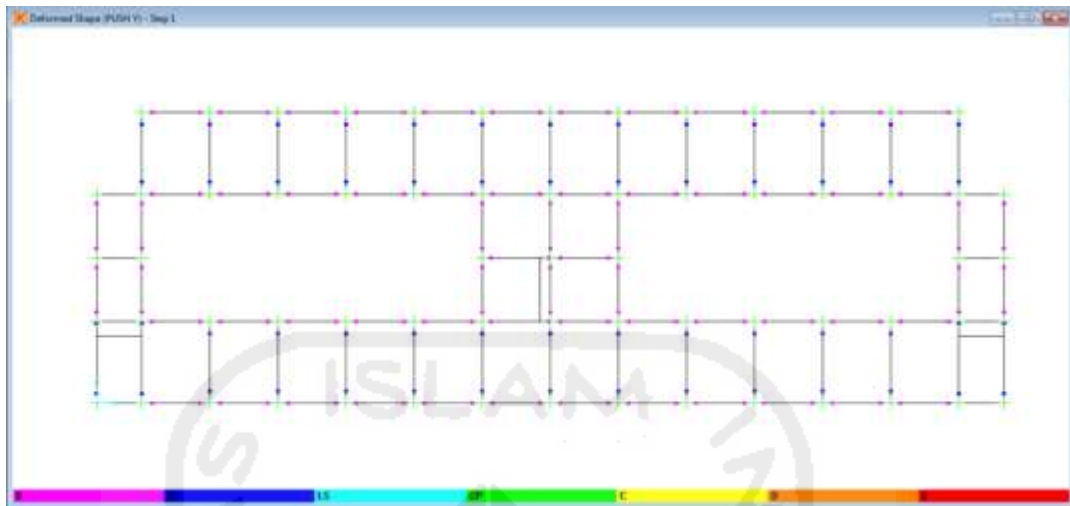
Gambar 5.60 Sendi plastis balok TB pushover arah y step 1
