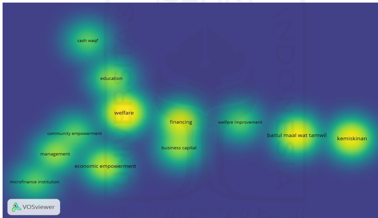
Gambar 7 Density Visualization
