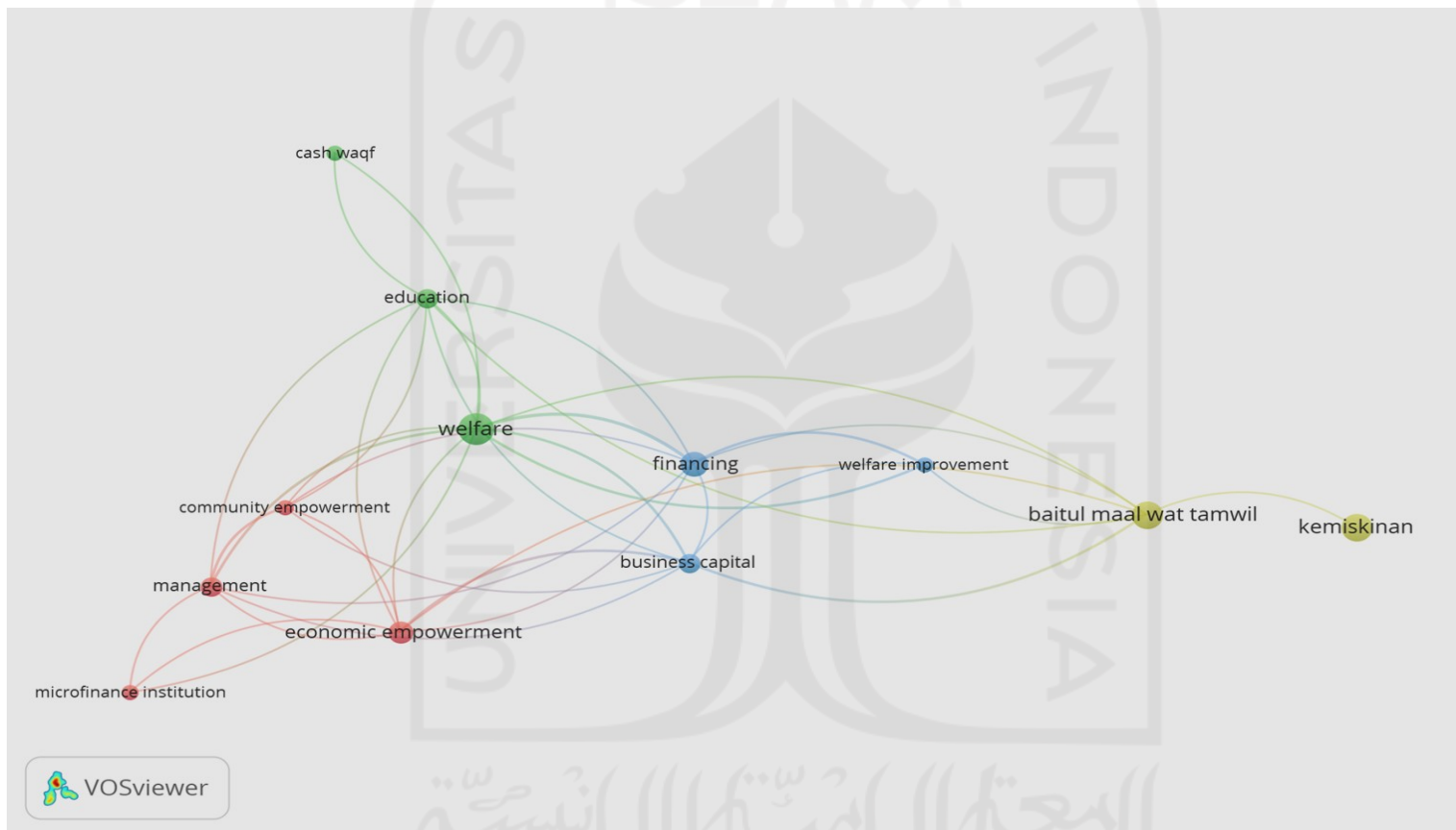
Gambar 5 Network Visualization
