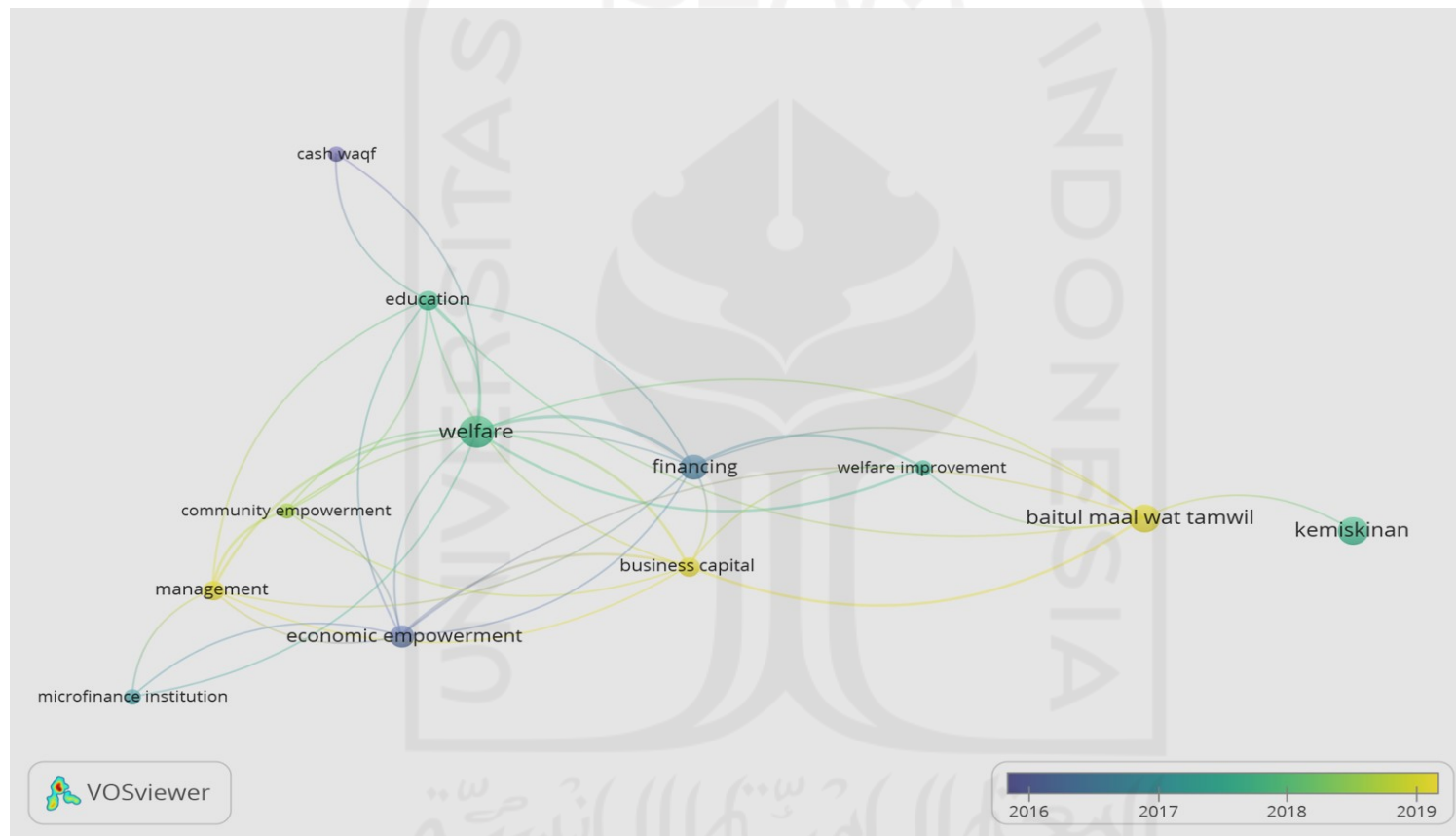
Gambar 6 Overlay Visualization
