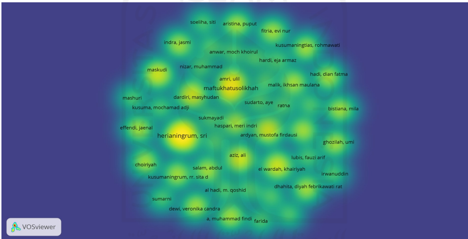
Gambar 4 Density Visualization
