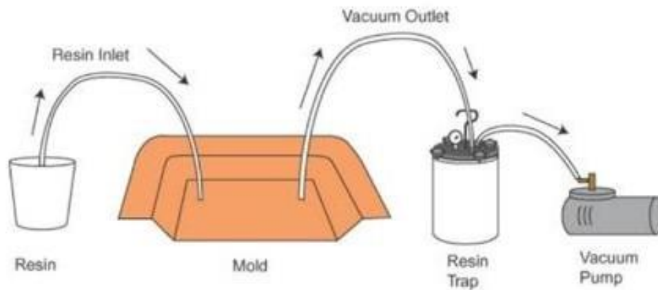
Gambar 2. 5 Skema Vacuum Infusion
