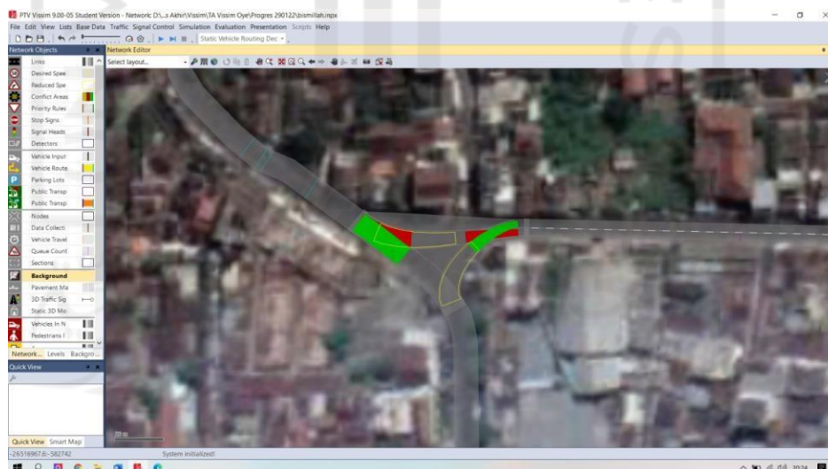
Gambar 5.22 Pengaturan Reduced Speed Areas
