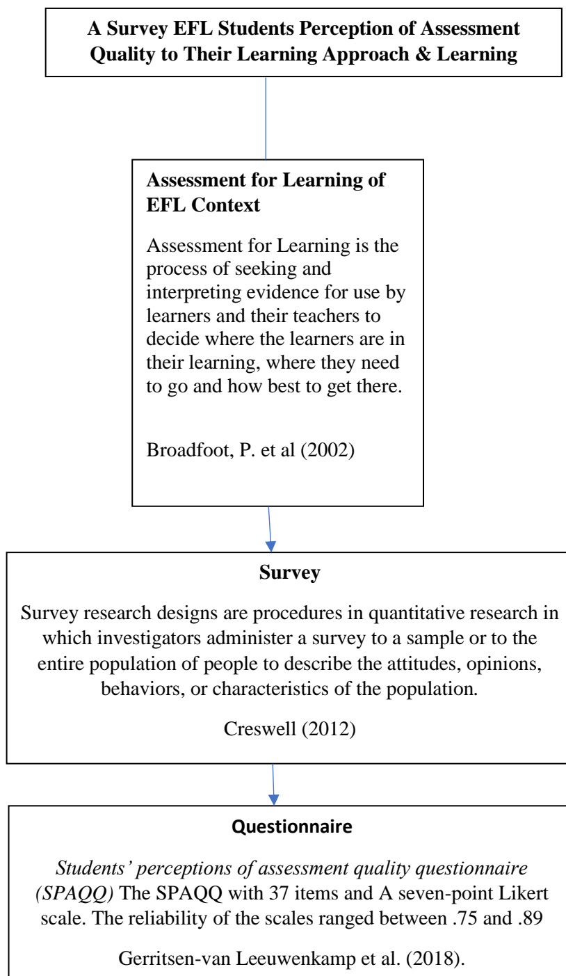
Figure 2.1 Theoretical Framework
