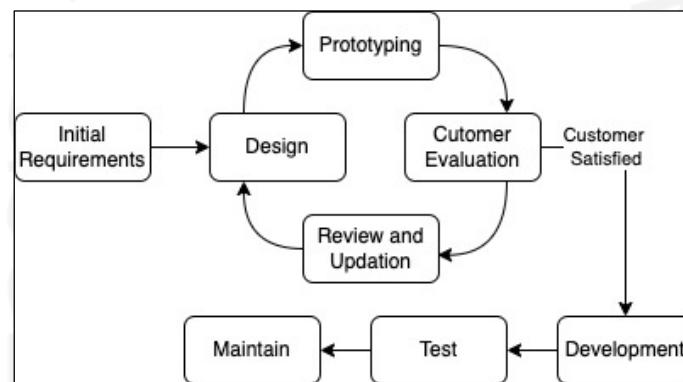
Gambar 2.3 Metode Prototyping
