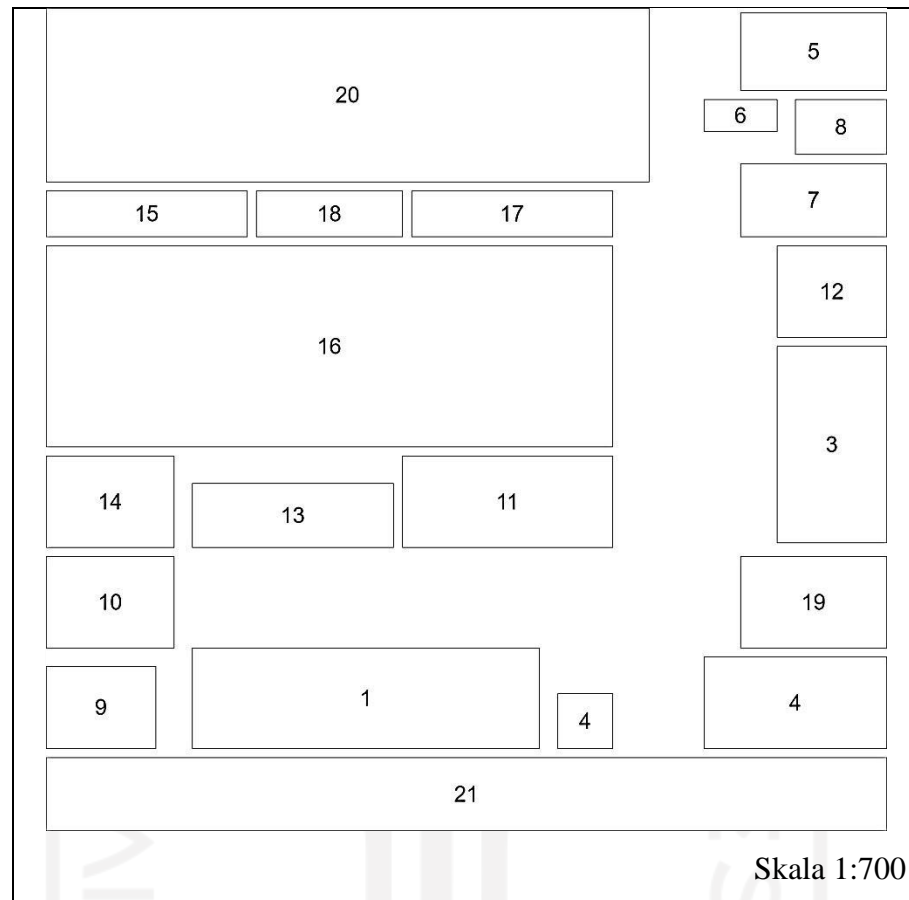
Gambar 4.1 Lay Out Pabrik VCO
