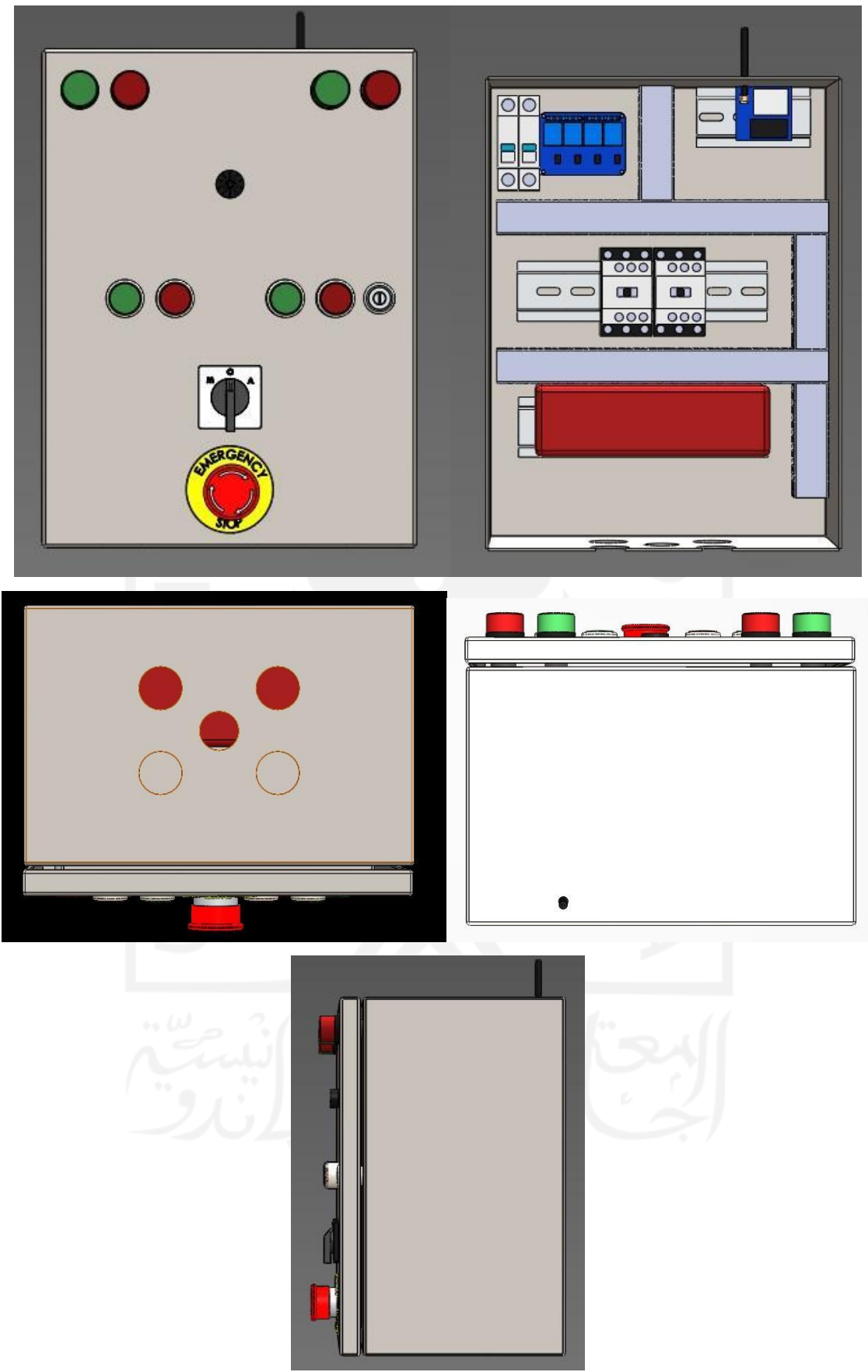
Gambar 3.4. Desain layout panel 3D
