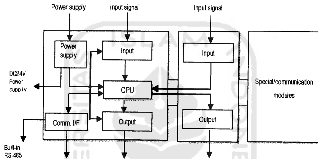
Gambar 2.5 Bagian-bagian PLC
