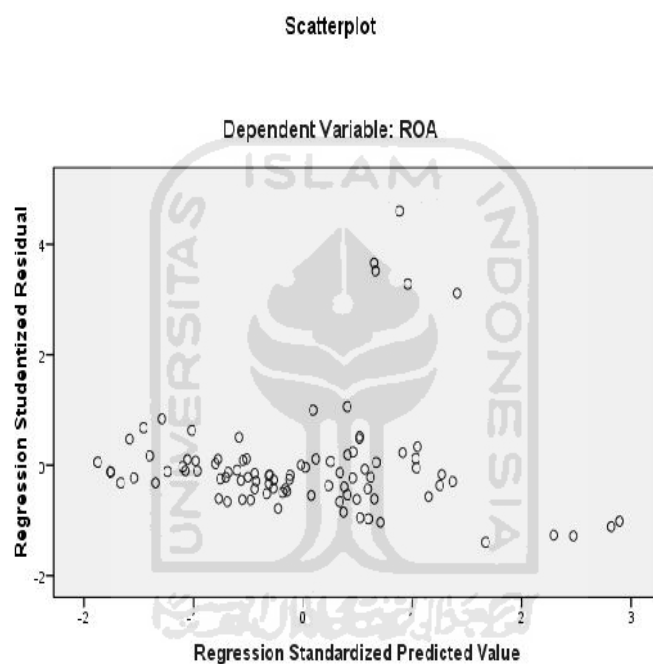
Gambar 4.2 Diagram Scatterplot
