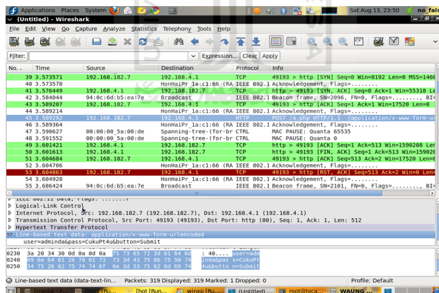
Gambar 4.16 Capture Wireshark
