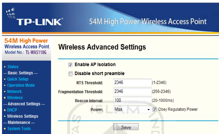
Gambar 4.32 AP isolation
