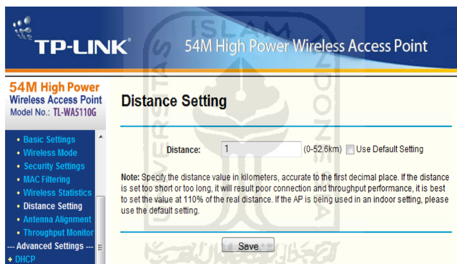
Gambar 4.31 Distance setting
