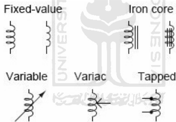
Gambar 2.6 Simbol-Simbol Induktor
