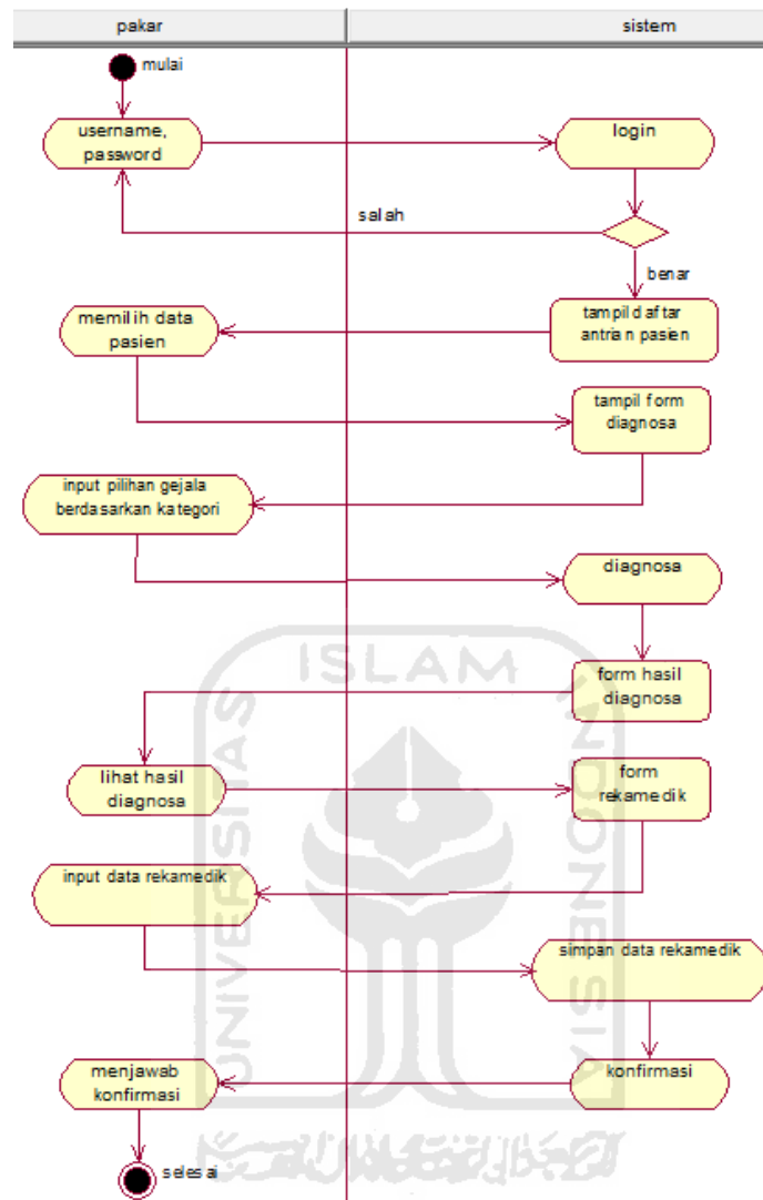
Gambar 4.9 Activity Diagram Diagnosa
