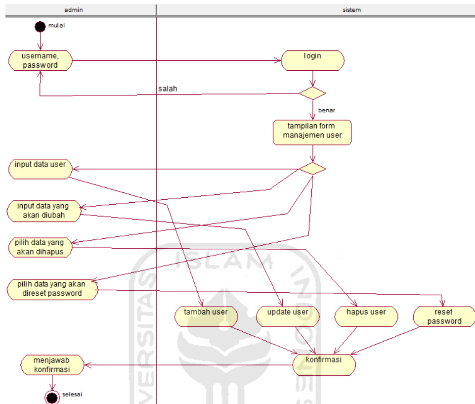
Gambar 4.3 Activity Diagram Manajemen User
