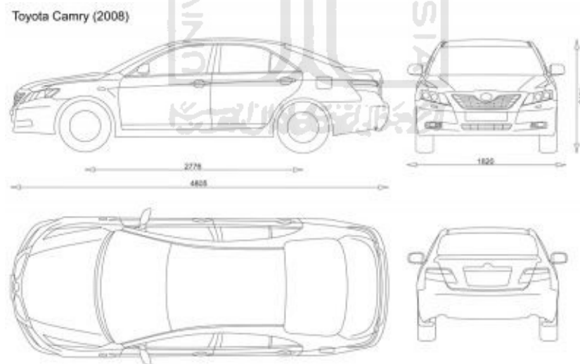
Gambar 3.2 Blueprint Mobil
