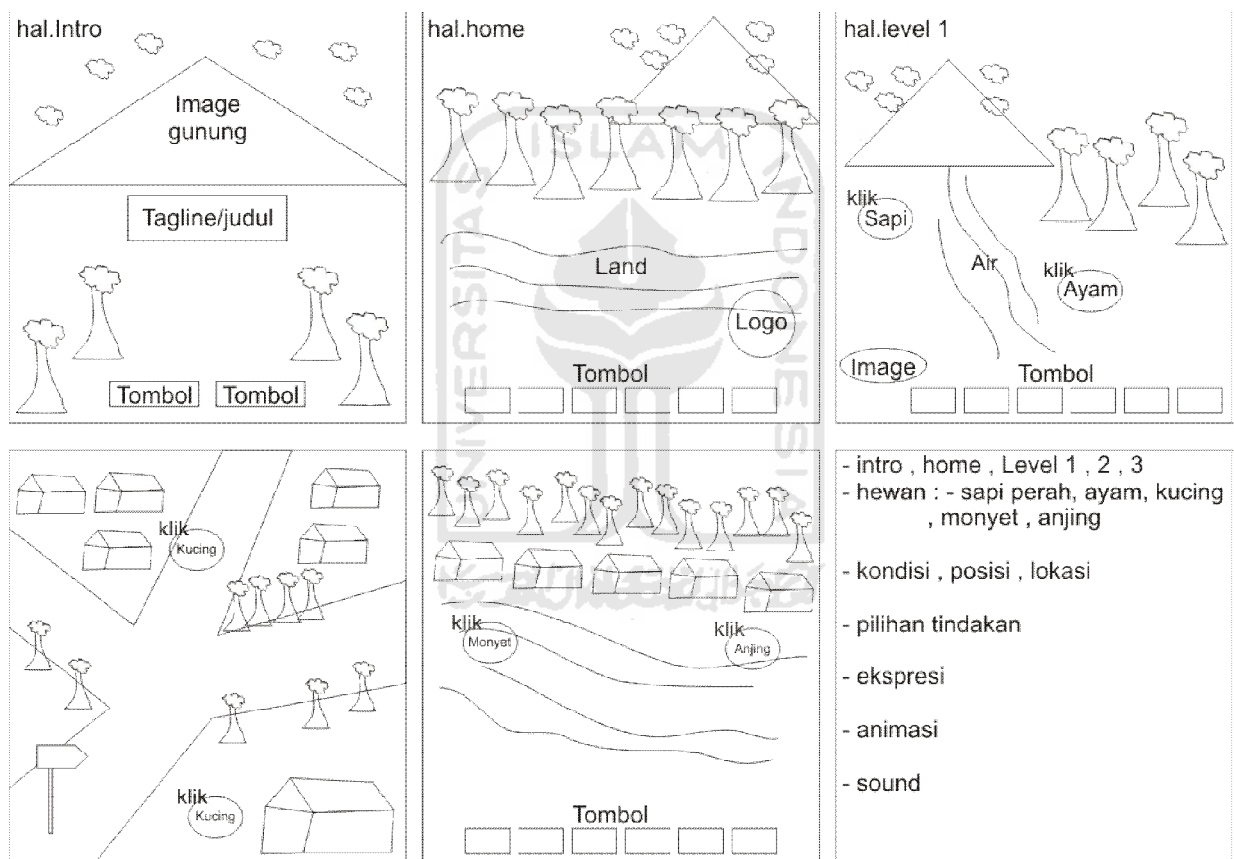
Gambar 3.1 Sketsa Storyboard
