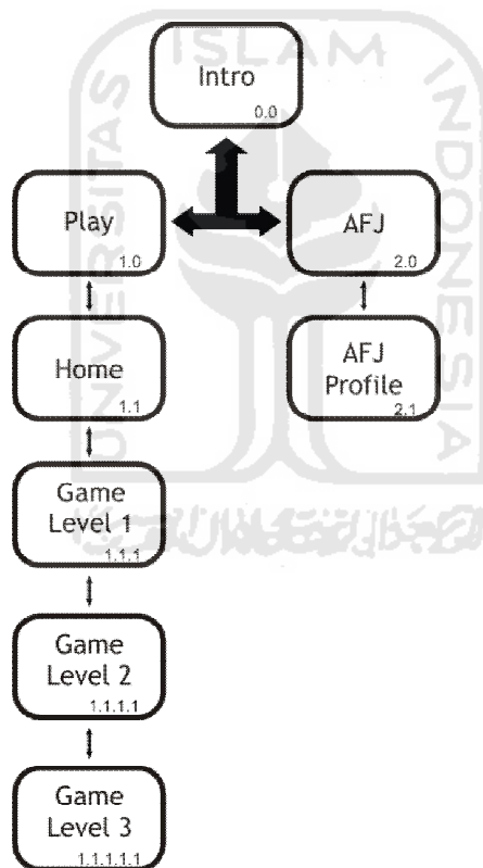
Gambar 3.2 Diagram hirarki
