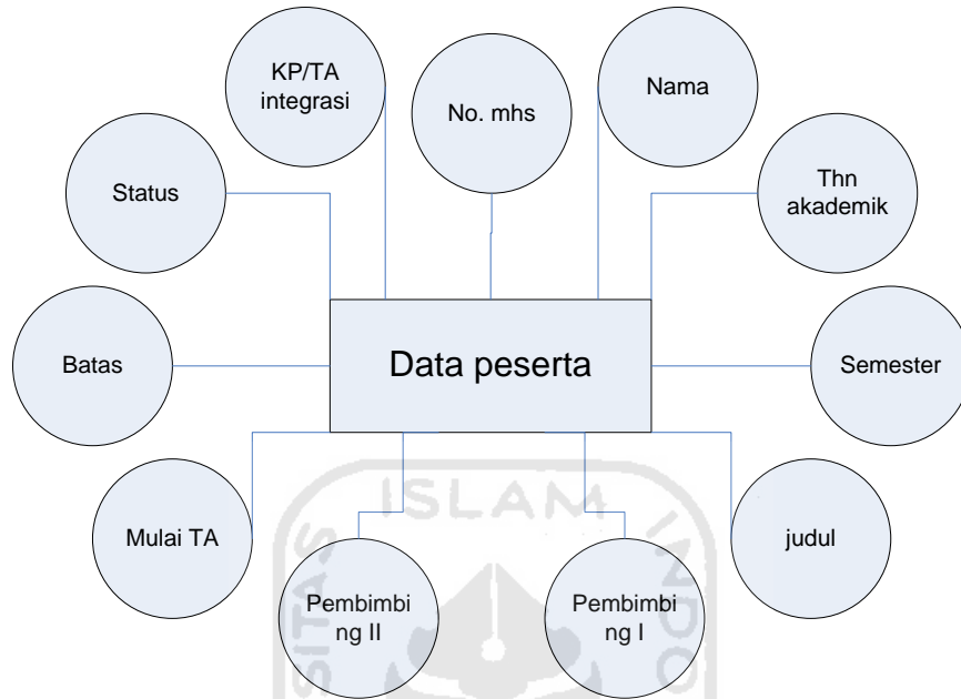
Gambar 4.16 Diagram ERD Data Peserta
