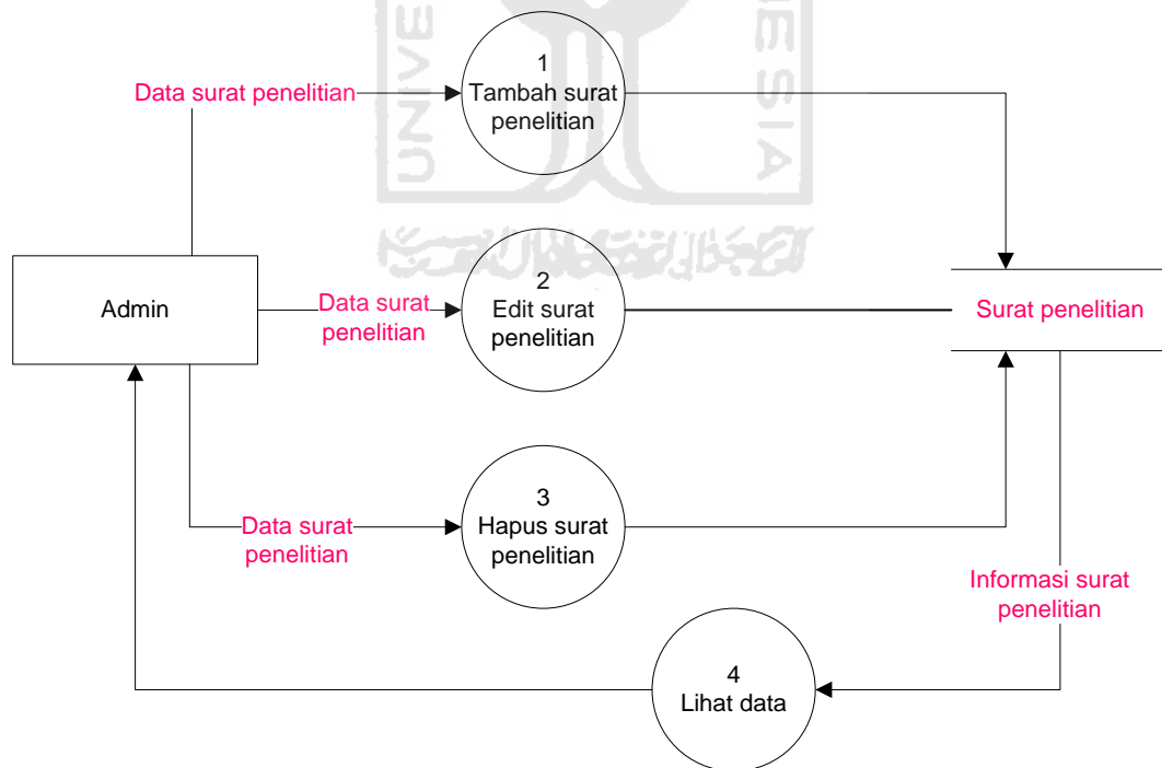
Gambar 4.40 DFD level-2 Surat Penelitian
