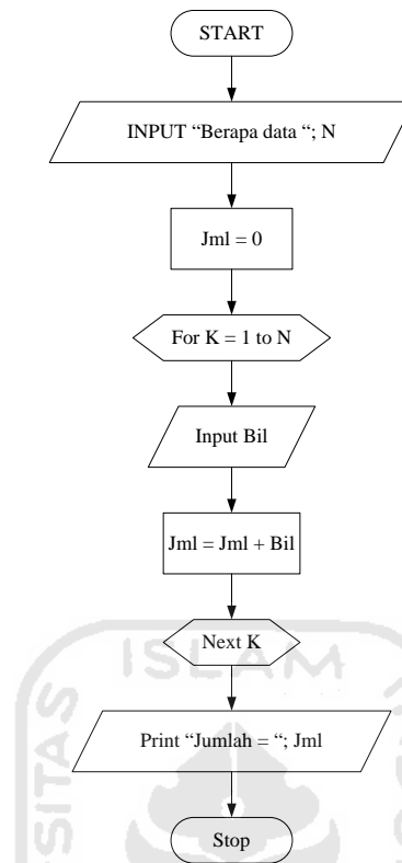
Gambar 2.7 Proses Detail Flowchart
