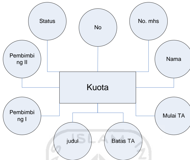
Gambar 4.18 Diagram ERD Kuota (b)
