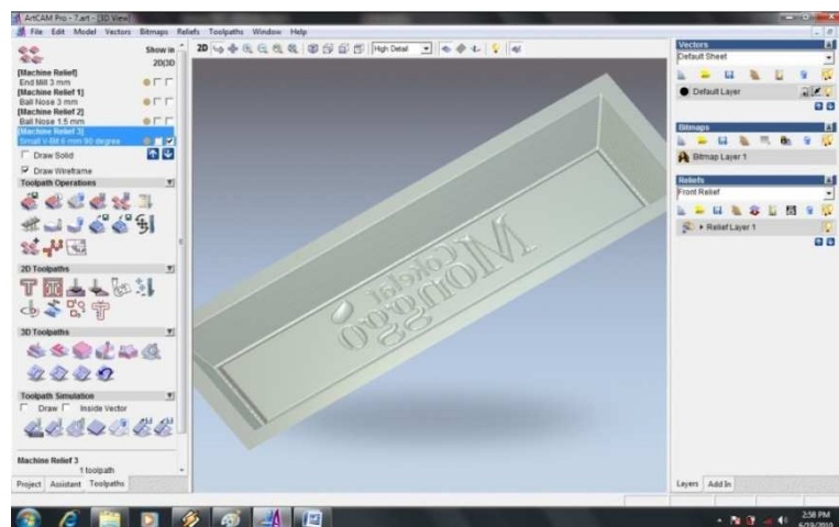
Gambar 3.11 Software ArtCam
