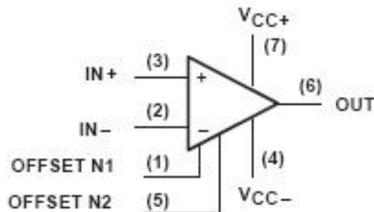
Gambar 2.5 Simbol penguat operasional
