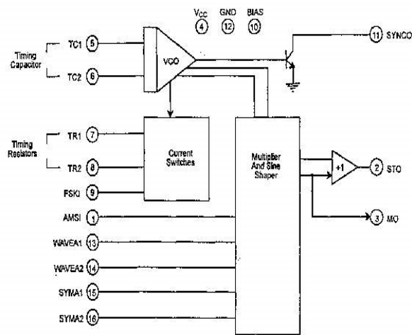
Gambar 2.4 Blok Diagram XR-2206
