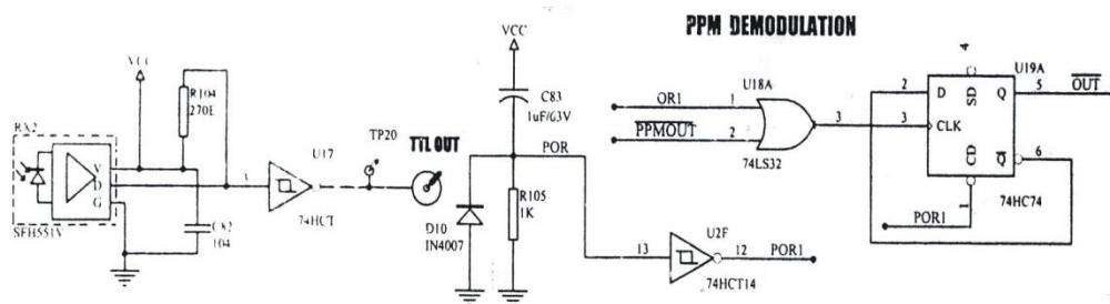
Gambar 3.10 Pulse Position Demodulation
