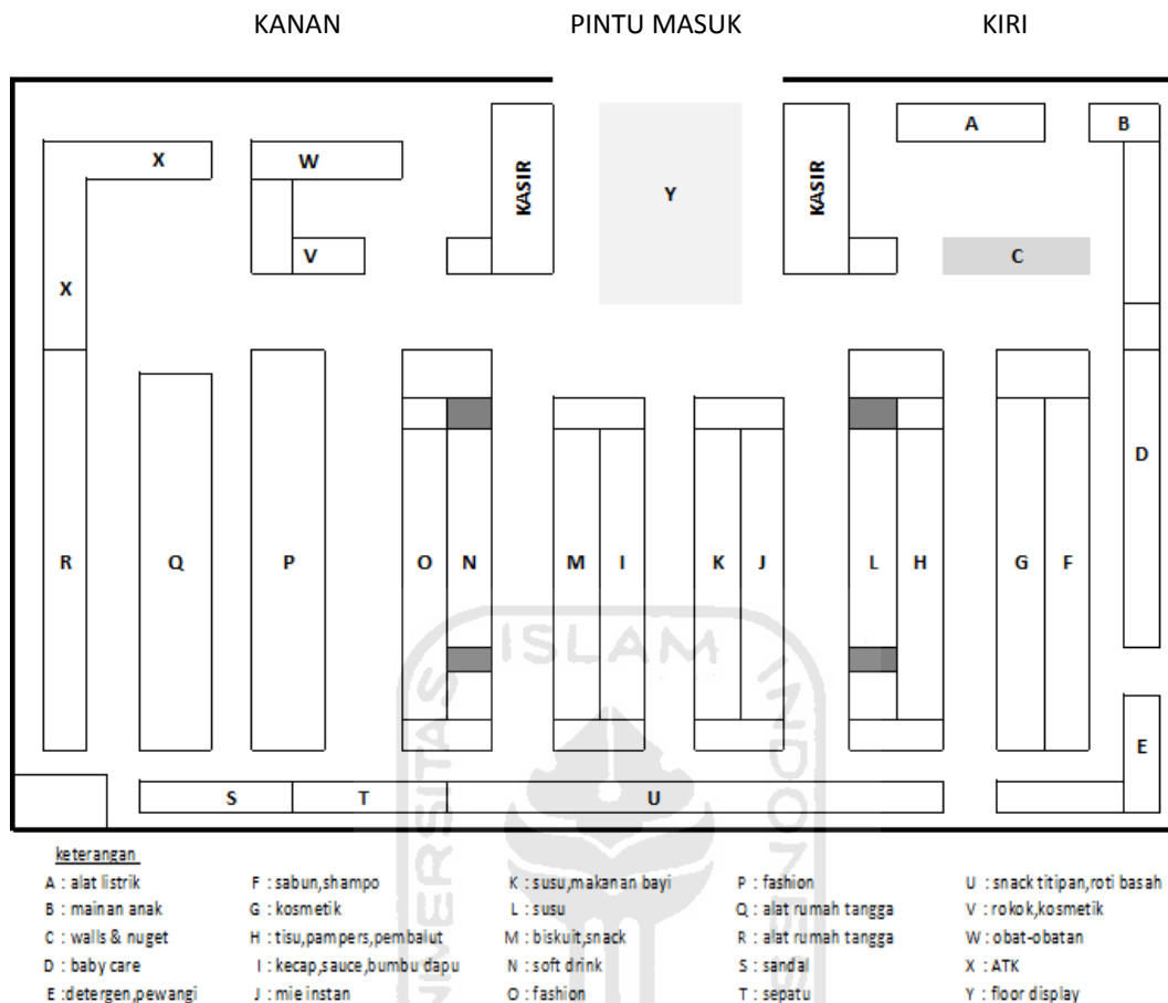
Gambar 5.3 Desain Layout berdasarkan Out put 1
