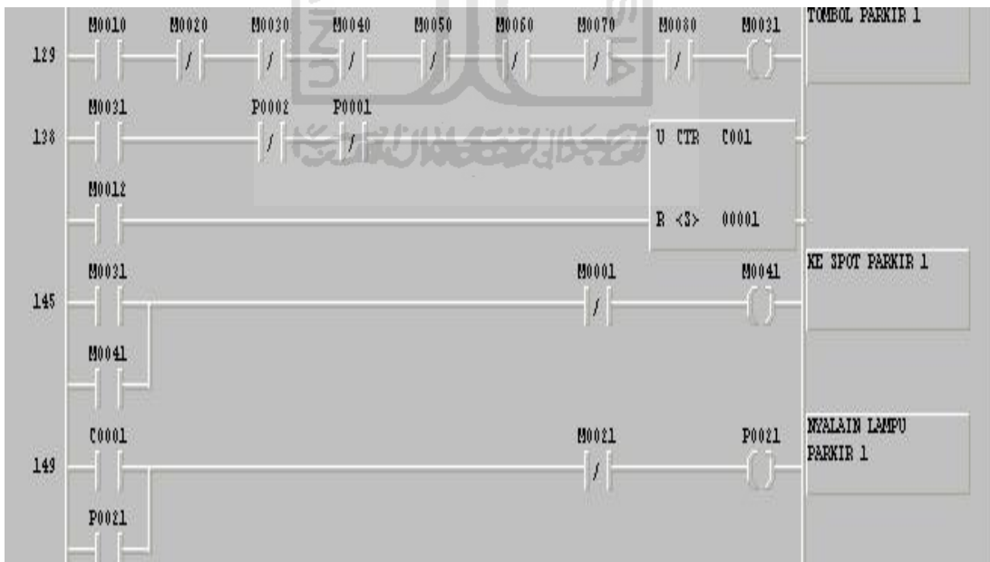
Gambar 3.11 Program Parkir 1
