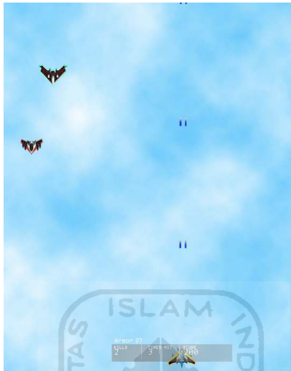
Gambar 4.2 Game
