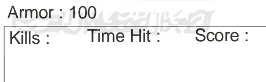
Gambar 3.3 Tampilan Score
