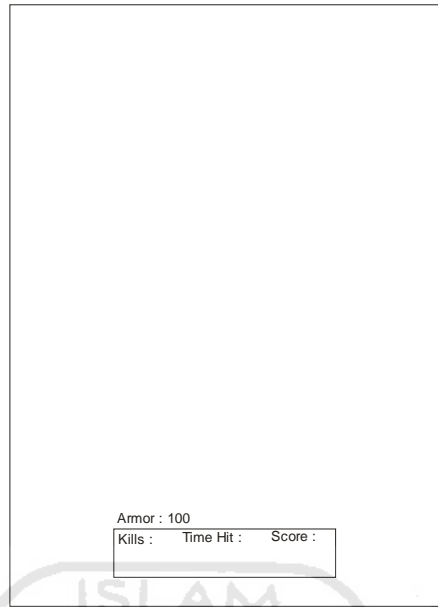
Gambar 3.2 Game
