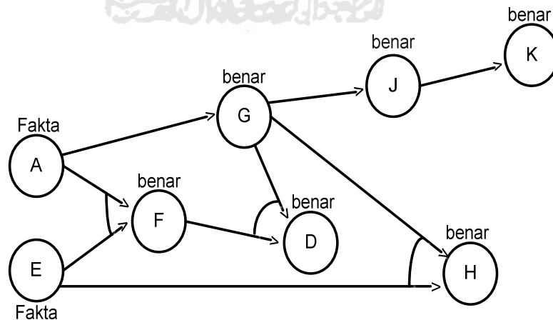
Gambar 2.1 Forward Chaining
