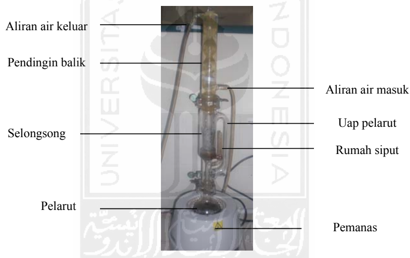
Gambar 4. Alat Soxhlet
