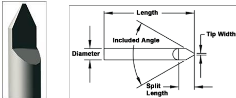
Gambar 4-6 Pahat Conical
