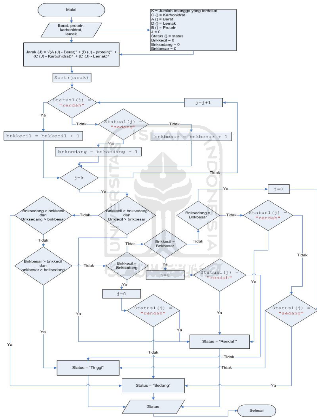
Gambar 2.2 Flowchart Metode K-NN
