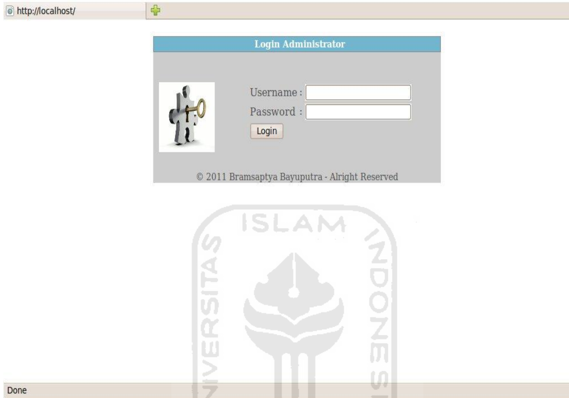
Gambar 4.1 Web Interface
