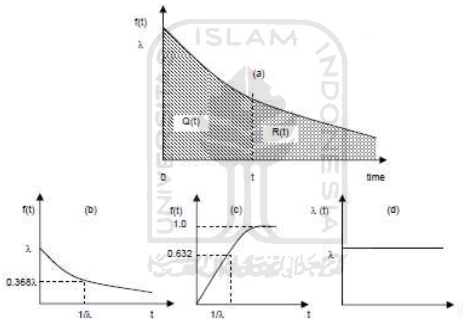
Gambar 2.3 Pola Distribusi Eksponensial a) F(t) dan R(t) ; b) Failure; c) Cumulative Failure Distribution ; d) Hazard Rate
